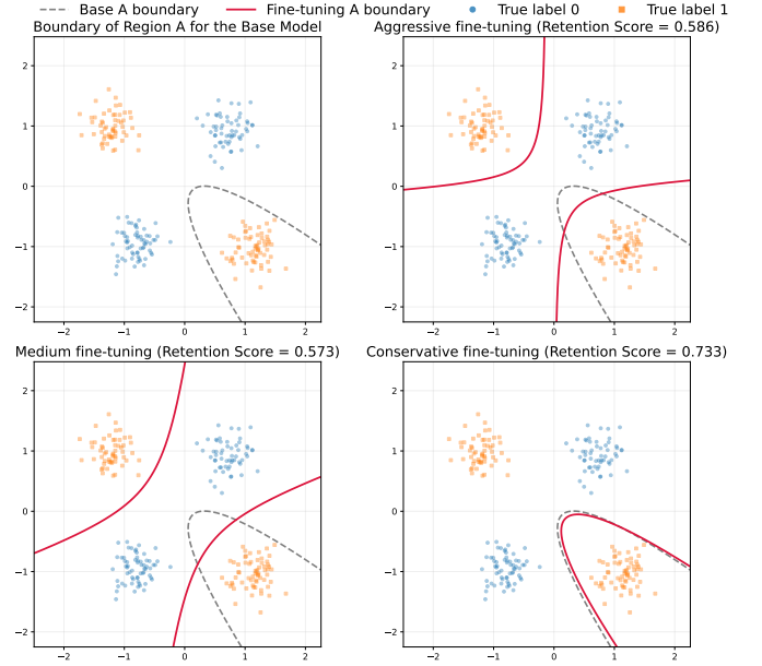
Fig. 10. Visualization of the retention of the dominant sufficiency–necessity explanation structure under fine-tuning on a synthetic dataset.
