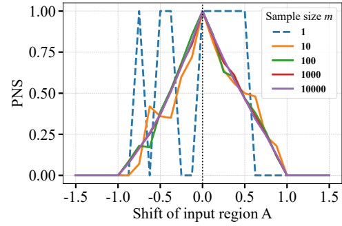
Fig. 3. Monte Carlo estimates of \text{PNS}(A, B^*) as the continuous input region A is shifted away from an optimal reference region A^* under different sample sizes m .
