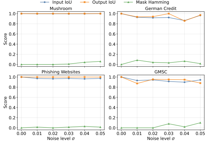
Fig. 9. Robustness analysis of SNRE explanations under increasing training input noise across four datasets, measured by Input IoU, Output IoU, and Mask Hamming.
