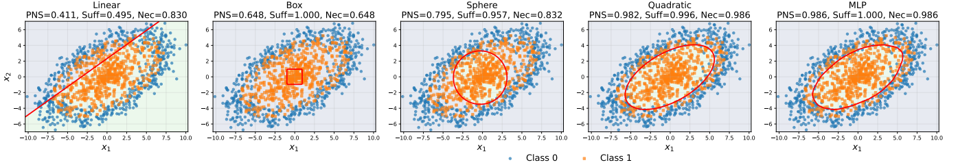
Fig. 7. Comparison of input region shapes from different parameterizations. A 2D example shows that linear, box, and spherical shapes are too rigid to fit the data, while an MLP learns a complex, irregular boundary. The quadratic hypersurface forms a regular ellipse, best balancing geometric expressiveness and interpretability.
