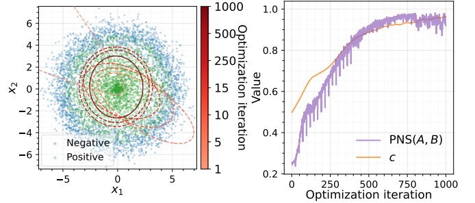
Fig. 5. Toy example for joint learning of an input-output region pair (A, B) with SNRE. Left: snapshots of the learned input region A , represented by the quadratic boundary g(\mathbf{x}) = 0 , across optimization iterations. Colors indicate snapshot iterations, with dashed contours for intermediate snapshots and a solid contour for the final one. Right: optimization trajectories of the region-level \text{PNS}(A, B) and the output region parameter c defining B = [c, 1] over optimization iterations.
