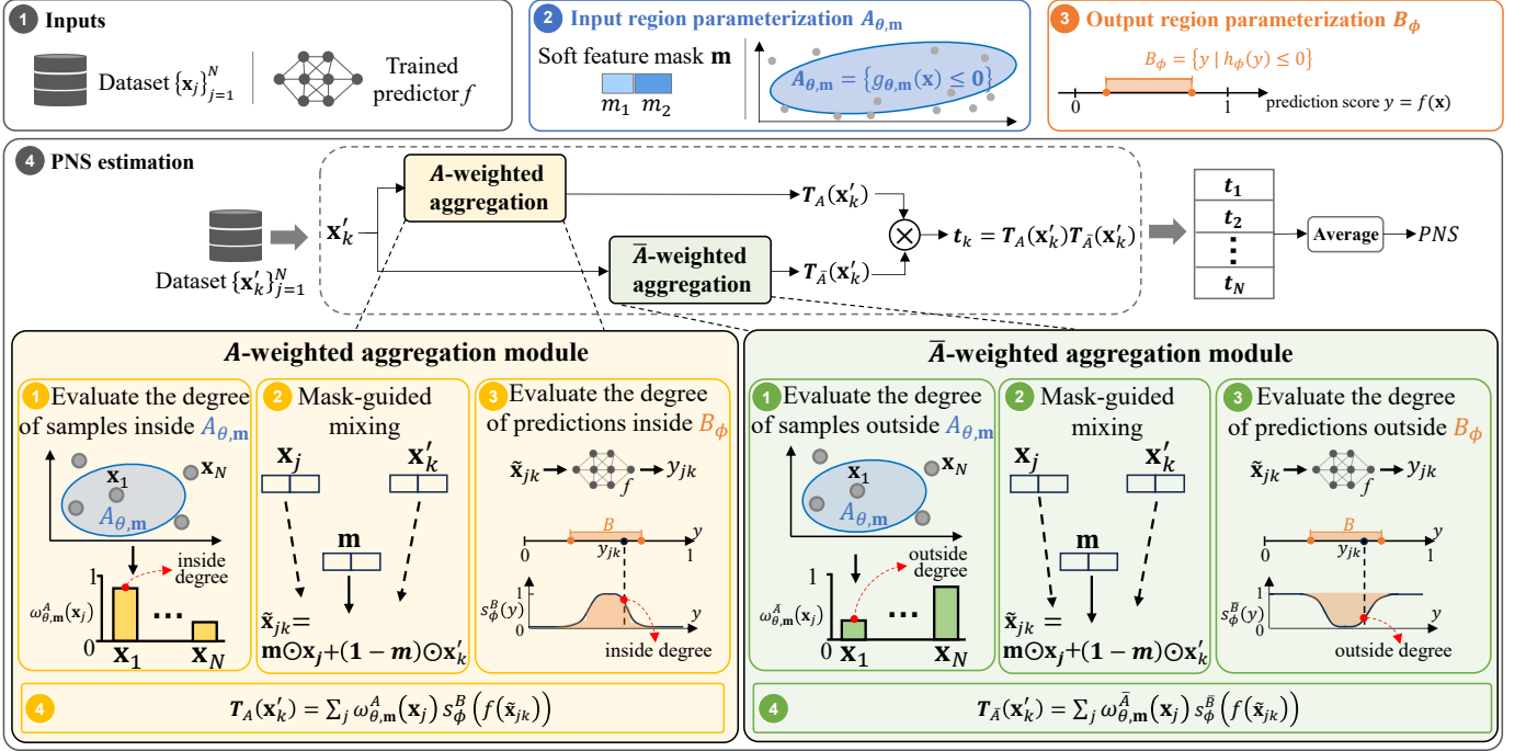
Fig. 4. SNRE framework for learning sufficient-and-necessary input-output region pairs. SNRE first parameterizes the input region A_{\theta, m} and output region B_{\phi} , and then estimates PNS through outer marginalization and two parallel weighted aggregation modules. The A -weighted module evaluates how strongly inputs inside A_{\theta, m} induce predictions inside B_{\phi} , while the \bar{A} -weighted module evaluates how strongly inputs outside A_{\theta, m} induce predictions outside B_{\phi} . The final PNS objective is obtained by averaging the product of the two aggregation terms over the training samples used for marginalization.
