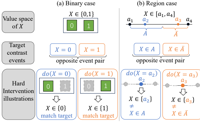
Fig. 2. Illustration of why hard interventions fail for region-level events. In the binary case, hard interventions exactly match the two opposite target events. In the region case, hard interventions collapse the value space to singleton events and therefore cannot realize the contrast between X \in A and X \in \bar{A} .
