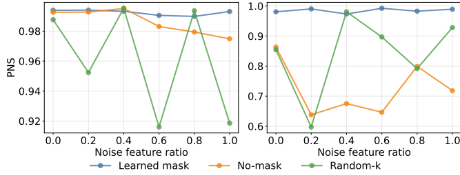
Fig. 8. PNS under different feature-mask strategies with increasing noise-feature ratios.
