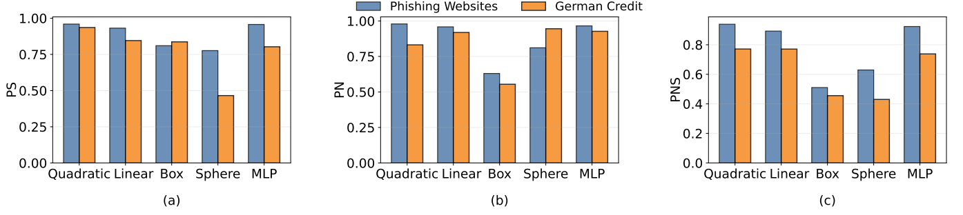
Fig. 6. Ablation on input-region parameterization. We compare five region families, including linear, box-shaped, spherical, quadratic, and MLP-based implicit boundaries, on Phishing Websites and German Credit. The results are reported in terms of PN, PS and PNS. Quadratic parameterization achieves a favorable balance between expressive power and explanation quality across datasets.
