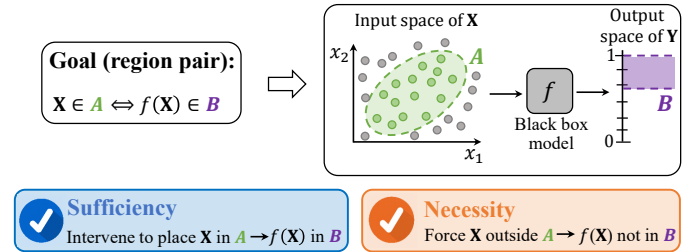
Fig. 1. Conceptual comparison between conventional rule/region explanations and SNRE (Sufficient and Necessary Regional Explanations). Conventional rule/region explanations identify an input-side region A associated with a target prediction, yet samples outside A may yield the same output. SNRE learns an input-output region pair (A, B) by contrasting in-region and out-of-region interventions, capturing both A \rightarrow B and \bar{A} \rightarrow \bar{B} .
