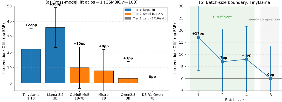
Figure 3: Applicability map for Intervention C. (a) Cross-model lift at bs=1 for six models (including the MoE architecture OLMoE), coloured by tier (Table 12): Tier 1 (Llama family, large lift), Tier 2 (non-Qwen 7B, Qwen-3B, and OLMoE-MoE; small but positive), Tier 3 (Qwen BF16-saturated). Error bars are 95% CIs on the paired lift. (b) Batch-size scaling on TinyLlama-1.1B (Appendix VIII): the lift holds at bs \leq 4 (green band, where C alone is sufficient in this experiment) and vanishes at bs \geq 8 (grey band, where composition with global FP32 compute recovers a small positive lift). Together, the panels summarise the tested (model, bs) region in which the lm_head -only intervention helps.
