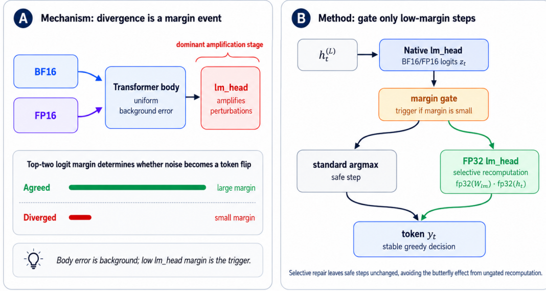
Figure 2: Mechanism and method. (A) Cross-precision divergence is a margin event : BF16 and FP16 accumulate uniform background error through the transformer body, and the lm_head —the dominant amplification stage—turns that error into a token flip only when the top-two logit margin is small. Prompts with a large margin agree across precisions; prompts with a small margin diverge. (B) Our method gates on this margin: the native (BF16/FP16) lm_head logits z_t are computed first, and only when the margin is small does the gate trigger a selective FP32 lm_head recomputation ( \text{fp32}(W_{lm}) \cdot \text{fp32}(h_t) ); large-margin (safe) steps take the standard argmax unchanged. Selective repair ( \sim 1.4\% of steps) leaves safe steps untouched, avoiding the butterfly effect of ungated recomputation.
