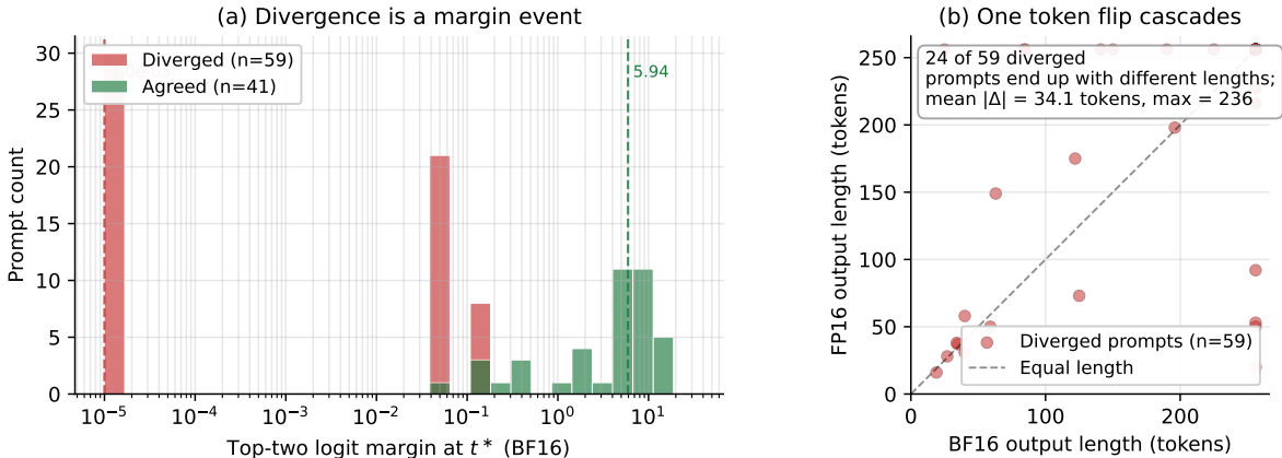
Figure 1: Two empirical facts that shape this paper (TinyLlama-1.1B, GSM8K, BF16 vs. FP16 greedy decoding, n = 100 ). (a) Distribution of the top-two logit margin at the measurement step t^* , for prompts whose outputs diverge (red) and for matched agreed controls (green). The two groups are bimodal across more than five orders of magnitude. DIVERGED median \approx 10^{-5} , with 30/59 exactly at 0 (perfect BF16 ties); AGREED median \approx 5.9 . Divergence is a margin event at the lm_head , not an error-magnitude event in the transformer body. (b) Sequence-length scatter of BF16 vs. FP16 outputs on the 59 DIVERGED prompts. A single token flip typically cascades into trajectory-level divergence: 24/59 prompts end up with different lengths, with a mean length difference of 34 tokens and maximum difference of 236 tokens.
