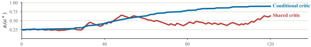
Figure 2: A sample trajectory of Algorithm 1 under the shared and the conditional value baseline ( q_E = q_H = \frac{1}{2} , r_E = (1, 0.8, 0.6) , r_H = (0.4, 0.2, 0) , \eta = 0.5 ): the conditional path increases at every update after an early transient, while the shared path keeps stepping backward.
