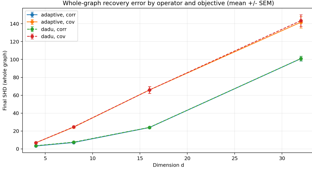
Figure 6: Whole-graph SHD by graph size, operator, and objective (mean \pm standard error, 16 reps per point, both densities and all three noise scales pooled). The DADU and ADAPTIVERELAX curves are visually indistinguishable within each objective at every d , making the point Table 6 makes locally—ADAPTIVERELAX’s gains are concentrated on the single wrongly-forbidden edge—visible at the level of the whole graph: relaxation operator has no detectable effect on SHD, while fitting objective has a large one.
