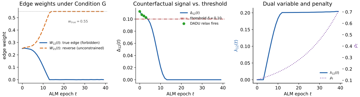
Figure 2: The early suppression trap on a fully controlled synthetic instance (Section 4.1), true edge 1 \rightarrow 2 with w_0 = 0.55 , the wrong-forbidden condition, \delta = 0.10 . Left: the forbidden true edge W_{12}(t) collapses to zero by epoch 14 while the unconstrained reverse edge W_{21}(t) grows to the same magnitude as w_0 —Lemma 1’s tie appearing inside a live optimization trajectory. Center: the counterfactual signal \Delta_{12}(t) against the threshold \delta ; green markers show where DADU’s relax branch fires, all early, before the reverse edge has taken over the fit. Right: the dual variable \lambda_{12}(t) and penalty \rho_t ; \lambda_{12} plateaus once W_{12} \approx 0 , since tightening a weight already near zero adds almost nothing further.
