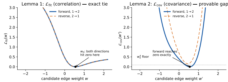
Figure 3: The two lemmas as one picture. Both panels plot fitting loss against a single candidate edge weight, at the true edge’s value w_0 = 0.55 ; the true (forward) direction is solid blue, the reverse direction dashed orange. Left (Lemma 1): under \mathcal{L}_{\text{fit}} , the two curves are the same function —they lie exactly on top of each other, both reaching zero at w_0 . Right (Lemma 2): under \mathcal{L}_{\text{cov}} , the two curves separate. The forward direction still reaches zero exactly at w_0 ; the reverse direction is bounded below by the w_0^4 floor at every candidate weight, including its own best case.
