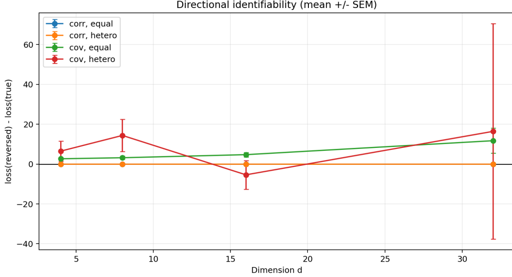
Figure 4: Directional loss gap by graph size, fitting objective, and noise type (mean \pm standard error, 96 trials per point: 16 reps \times 2 densities \times 3 noise scales, matching Table 2’s aggregation). Correlation (flat, both noise types) sits at zero across the entire range of d tested, visually confirming Lemma 1’s tie holds independent of graph size. Covariance under equal-variance noise (matching Lemma 2’s assumption) is positive and grows with d ; covariance under heteroscedastic noise is markedly less stable, consistent with the median-based reporting adopted in the text for that condition.
