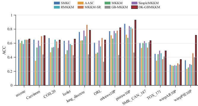
Fig. 2: ACC of eight methods on 12 datasets.
