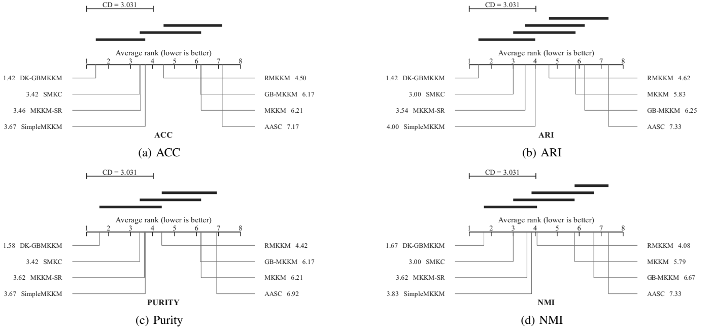
Fig. 5: Nemenyi critical-difference diagrams for four metrics. Lower average ranks indicate better performance; thick lines connect algorithms whose differences are not significant.
