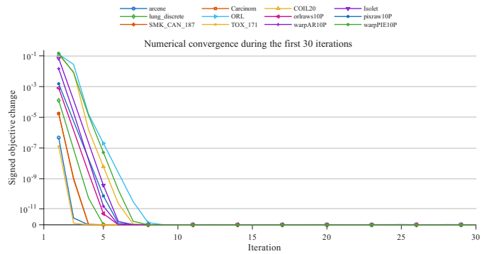
Fig. 3: Signed change in the DK-GBMKKM objective over the first 30 iterations on 12 datasets.
