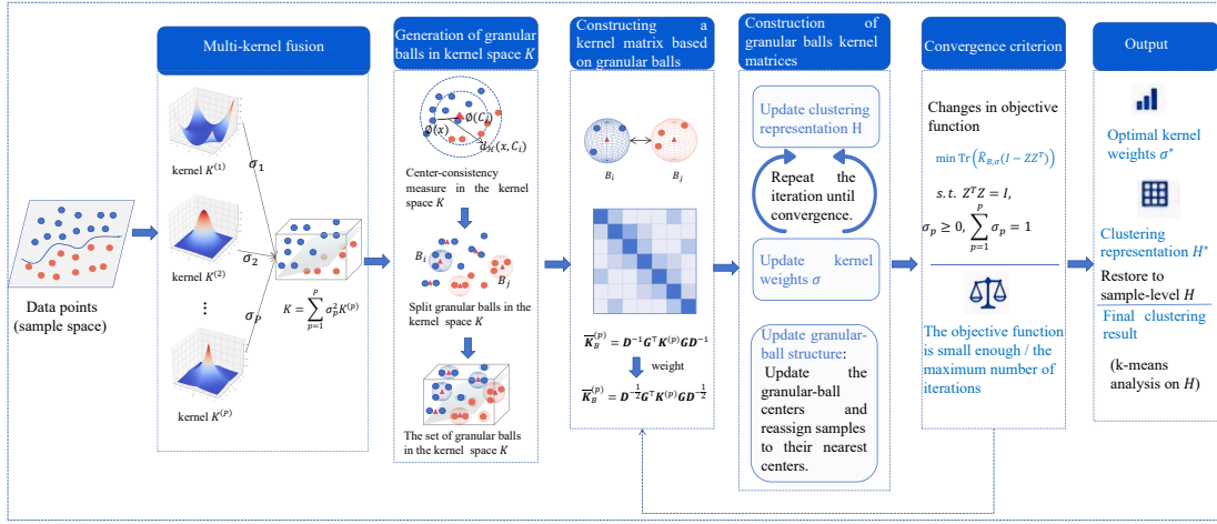
Fig. 1: Framework of DK-GBMKM.
