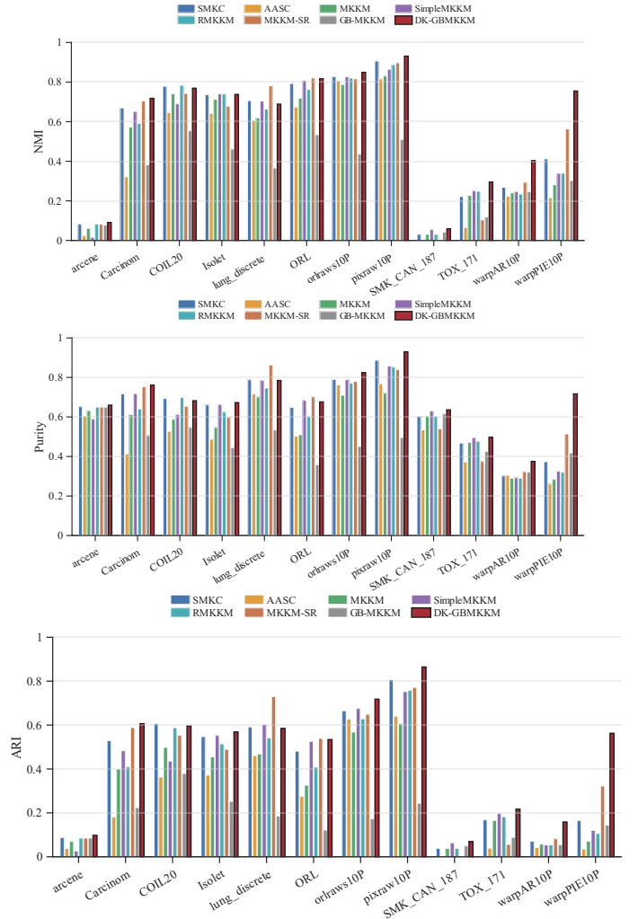
Fig. 4: Comparison of eight methods on 12 datasets: NMI (top), Purity (middle), and ARI (bottom).
