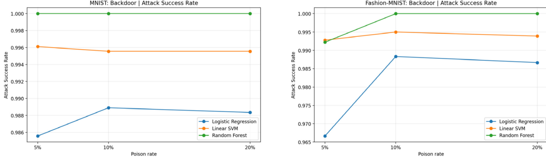
Figure 3: Backdoor attack success rate trends on MNIST and Fashion-MNIST.
