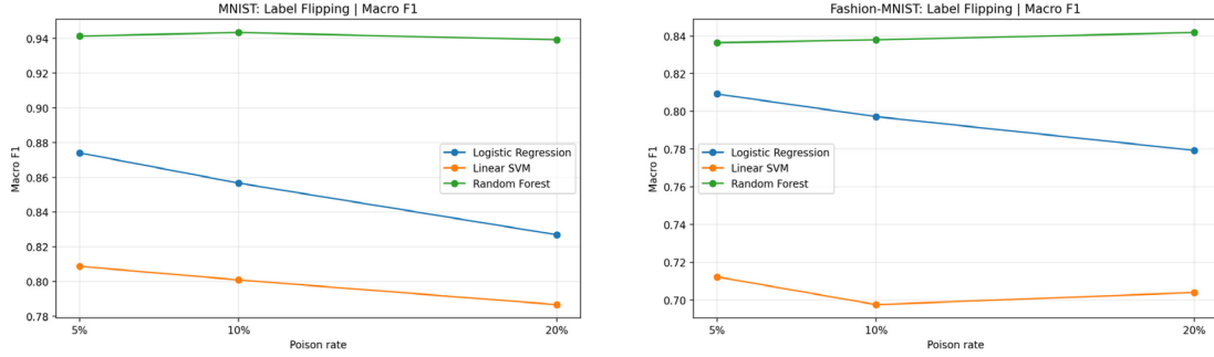
Figure 2: Label flipping macro-F1 trends on MNIST and Fashion-MNIST.
