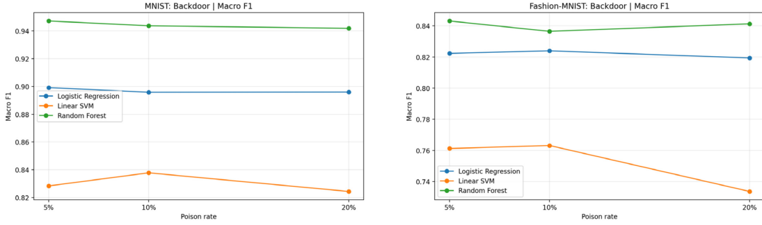
Figure 4: Backdoor macro-F1 trends on MNIST and Fashion-MNIST.
