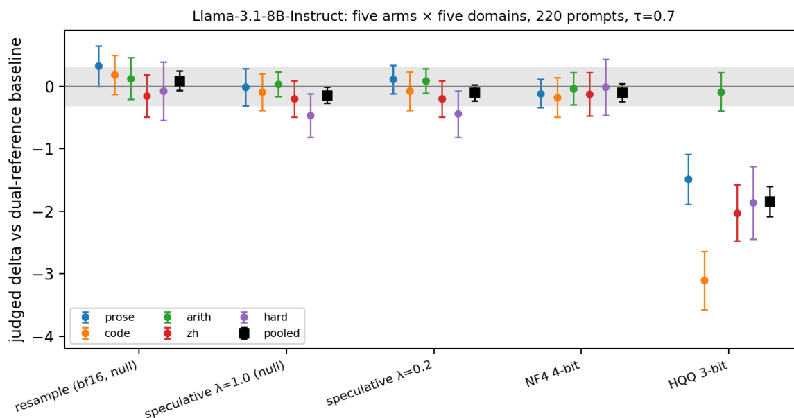
Figure 2. Judged delta with 95% confidence interval, Llama-3.1-8B.
