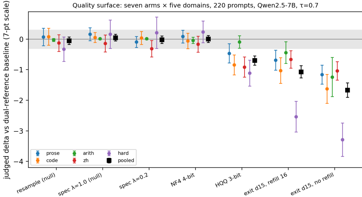
Figure 1. Judged delta with 95% confidence interval for each arm, by domain and pooled, Qwen2.5-7B. The grey band is the \pm 0.3 equivalence bound.
