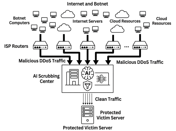
Fig. 1: General architecture of AI-assisted DDoS mitigation using traffic scrubbing centers and intelligent filtering.
