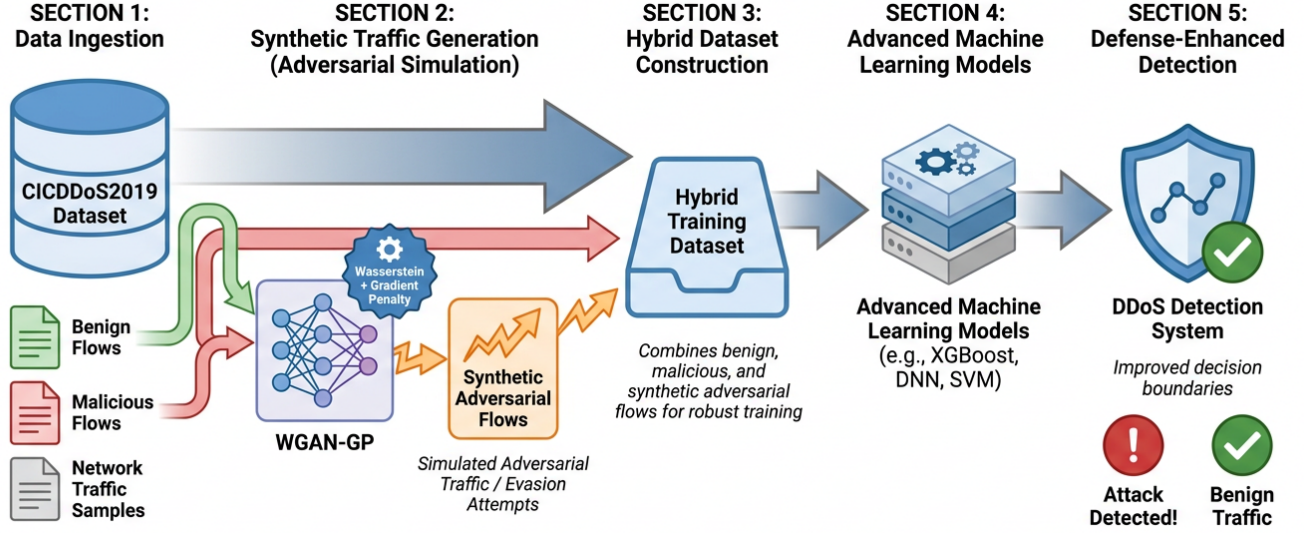
Fig. 2: DDoS Attack Detection Framework Integrating Generative Adversarial Modeling with Advanced Machine Learning
