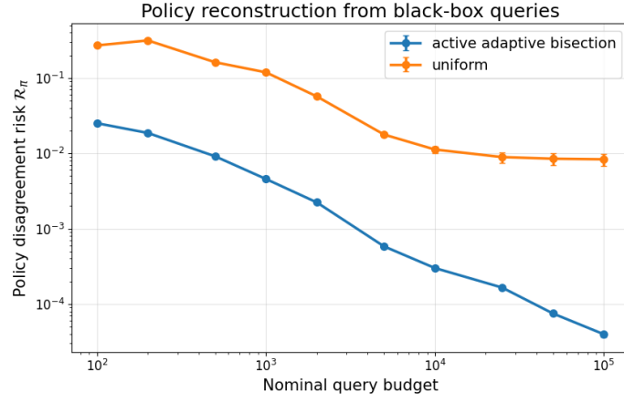
Figure 6: Policy reconstruction from black-box queries. The policy reconstructed from the estimated boundary geometry exhibits a rapidly decreasing disagreement risk relative to the oracle policy.
