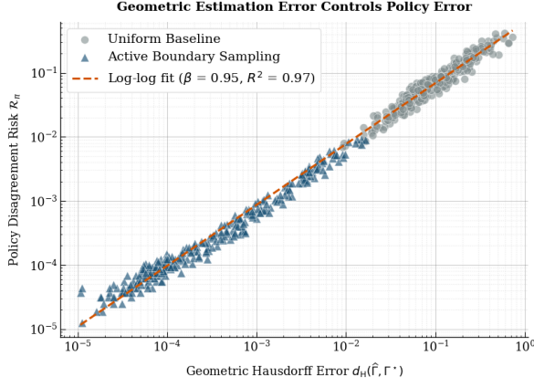
(a) Policy error versus geometric error.
