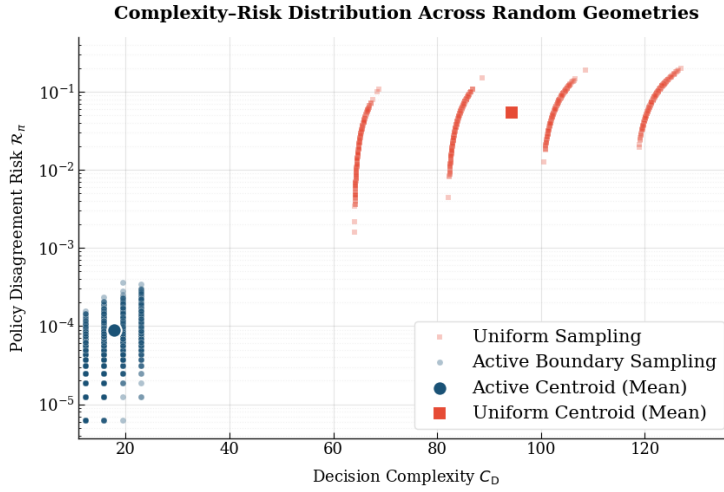
Figure 19: Complexity-risk joint distribution across random geometries. Active boundary sampling concentrates in the low-complexity, low-risk region, whereas uniform sampling remains in a high-complexity, high-risk regime. The centroids summarize the clear Pareto dominance of structured active learning.
