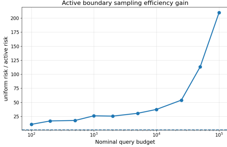
Figure 10: Active boundary sampling efficiency gain. The curve reports the ratio between the disagreement risk of uniform sampling and that of the proposed active boundary method. Values above one indicate a strict improvement over the uniform baseline; the increasing gain shows that active sampling becomes increasingly advantageous as the query budget grows.
