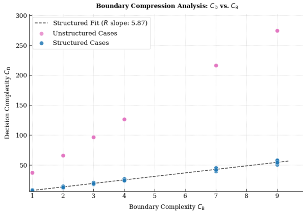
Figure 14: Boundary complexity versus decision complexity. Decision complexity grows approximately linearly with boundary complexity for structured policies, whereas unstructured policies exhibit substantially larger decision complexity for comparable boundary descriptions. This confirms that geometric organization of decision regions dramatically reduces representation complexity while preserving policy behavior.
