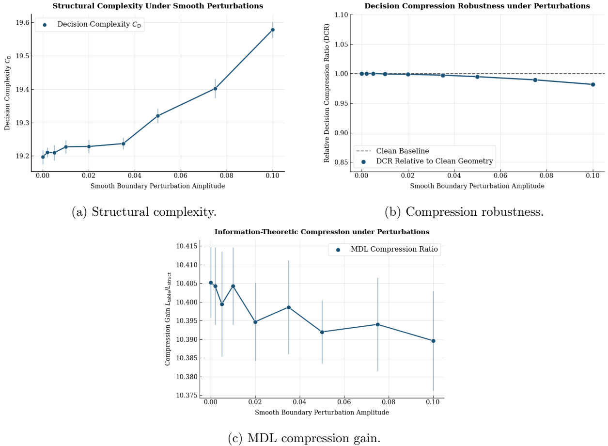
Figure 17: Robustness under smooth boundary perturbations. Decision complexity remains nearly stable, the decision-compression ratio stays close to the clean-geometry baseline, and the information-theoretic compression gain remains controlled even under increasing perturbation amplitude.
