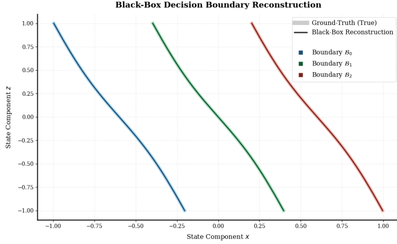
Figure 11: Black-box decision boundary reconstruction. Ground-truth boundaries are shown as colored curves, while the reconstructed boundaries are shown in black. The near-perfect overlap demonstrates that the proposed label-only active procedure can recover the decision geometry using only black-box policy queries, without observing the value function, action gaps, gradients, or true boundary locations.
