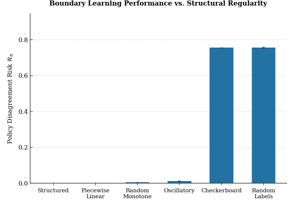
(b) Failure without structural regularity.
