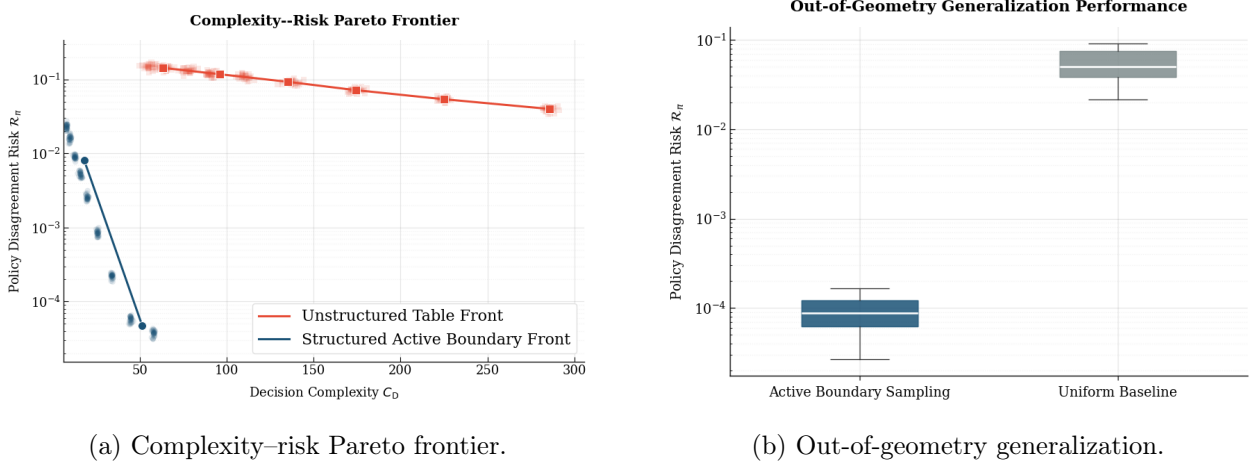
Figure 18: Complexity-risk trade-off and out-of-geometry generalization. Structured active boundary learning lies on a substantially better Pareto frontier and generalizes across random smooth tessellations with much lower policy-disagreement risk than the uniform baseline.
