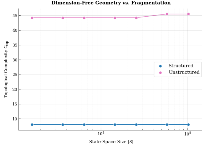
Figure 16: Dimension-free geometry versus fragmentation. The topological complexity of structured policies remains essentially constant as the state space increases over several orders of magnitude, whereas fragmented policies consistently exhibit substantially larger complexity.
