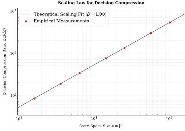
Figure 12: Scaling law for decision compression. The empirical decision-compression ratio \text{DCR}(n) increases proportionally to the size of the state space on logarithmic scales, closely matching the theoretical prediction with scaling exponent \beta \approx 1 . The near-perfect agreement between theory and experiments validates the asymptotic scaling law established in Section 6 and confirms that the compression gain grows predictably with problem size.
