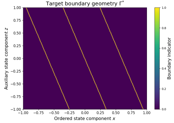
Figure 2: Target boundary geometry \Gamma^* . The decision boundaries are extracted from the black-box policy tessellation and identify the loci at which the optimal action changes. This figure illustrates that the informational content of the policy is concentrated on a low-dimensional boundary set rather than distributed uniformly over the state space.
