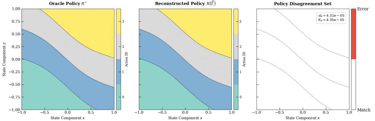
Figure 5: Policy reconstruction from the estimated decision boundary. The oracle policy \pi^* , the reconstructed policy \mathcal{R}(\hat{\Gamma}) , and the disagreement set show that the learned boundary induces an almost identical policy partition, with very small Hausdorff and policy-disagreement errors.
