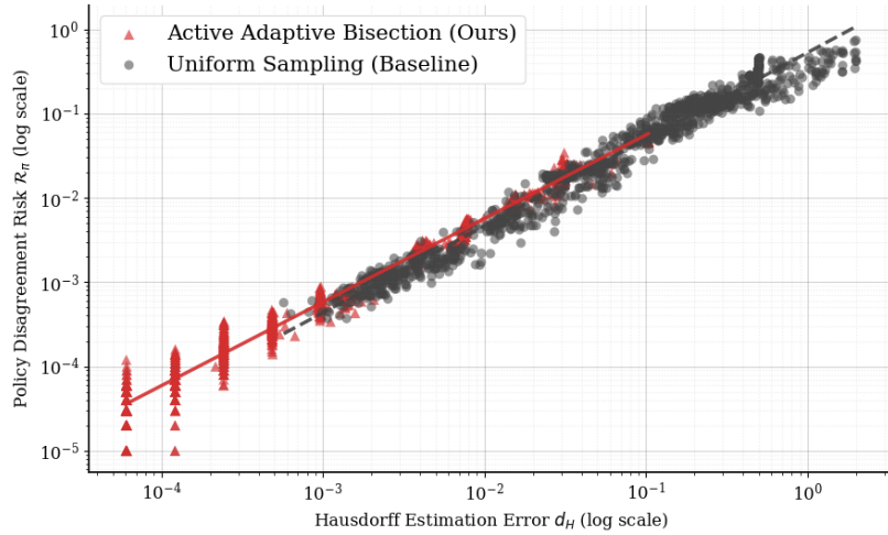
Figure 7: Geometric estimation error controls policy error. Each point corresponds to one seed–family–budget configuration. The log–log relationship shows that the policy disagreement risk scales with the Hausdorff boundary estimation error.
