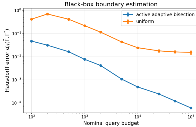
Figure 3: Black-box boundary estimation. The proposed active adaptive bisection procedure achieves substantially smaller Hausdorff boundary error than uniform sampling across all query budgets. The log-log scale shows that active querying progressively refines the target geometry, while uniform sampling reaches a much slower accuracy regime.
