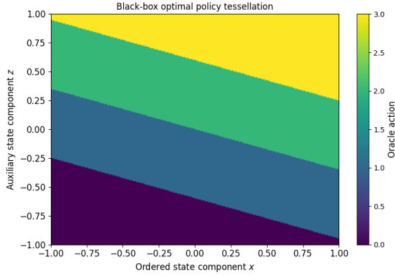
Figure 1: Black-box optimal policy tessellation. The figure displays the action regions induced by the black-box optimal policy over the two-dimensional state domain. Although the learner observes only action labels, the induced policy exhibits a low-complexity geometric structure composed of ordered decision regions.
