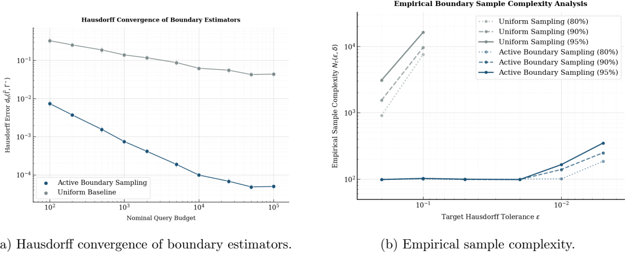
Figure 4: Boundary-estimation efficiency. Active boundary sampling achieves substantially faster Hausdorff convergence than uniform sampling while requiring fewer samples to reach the same geometric tolerance.
