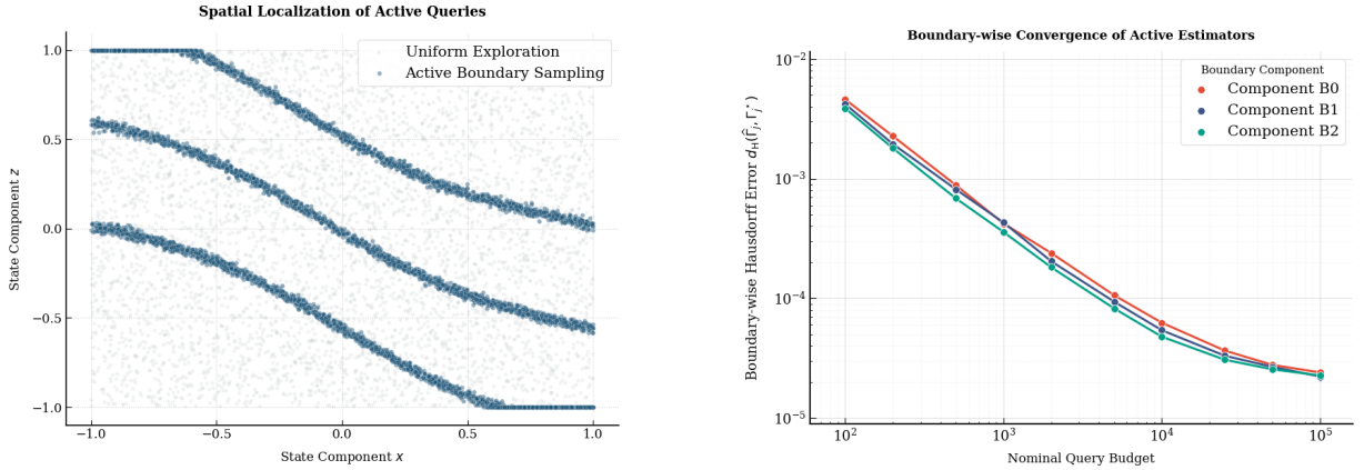
(a) Spatial localization of active queries.
