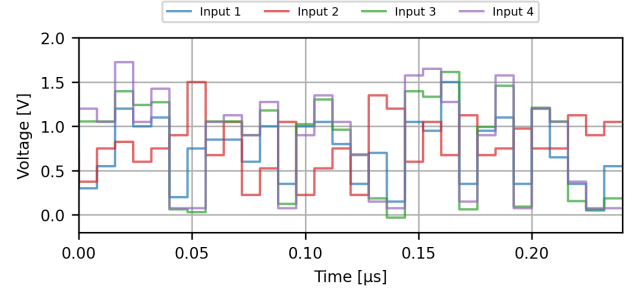
(a) Input waveforms
