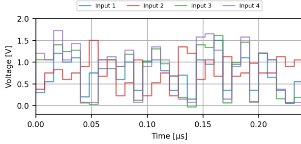
(a) Input waveforms
