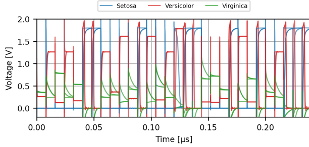
(c) Output waveforms (second-best validation circuit)
