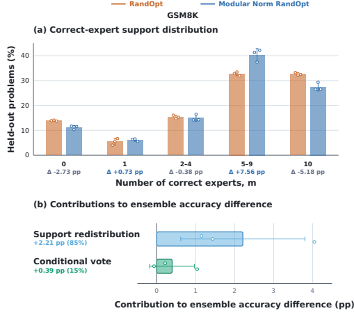
Figure 5: Selected-set support on GSM8K. Modular Norm RandOpt uses N = 25 , RandOpt uses N = 300 , and both use K = 10 . (a) Distribution of held-out evaluation problems by the number m of selected experts producing the gold answer. (b) Decomposition of the ensemble-accuracy difference into support redistribution and conditional voting. Bars show means, markers denote individual seeds, and error bars show mean \pm one sample SD over seeds 42–44, not confidence intervals.
