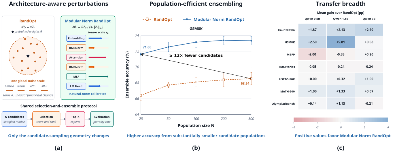
Figure 1: Modular Norm RandOpt enables architecture-aware, population-efficient ensembling. (a) Modular Norm RandOpt replaces isotropic perturbations with module-wise natural-norm and architecture-aware scaling, while keeping selection and ensembling unchanged. (b) On GSM8K with K = 25 , it exceeds RandOpt using \geq 12\times fewer candidates; error bars show one sample standard deviation over three seeds. (c) The calibrated geometry transfers across seven tasks and three Qwen model scales.
