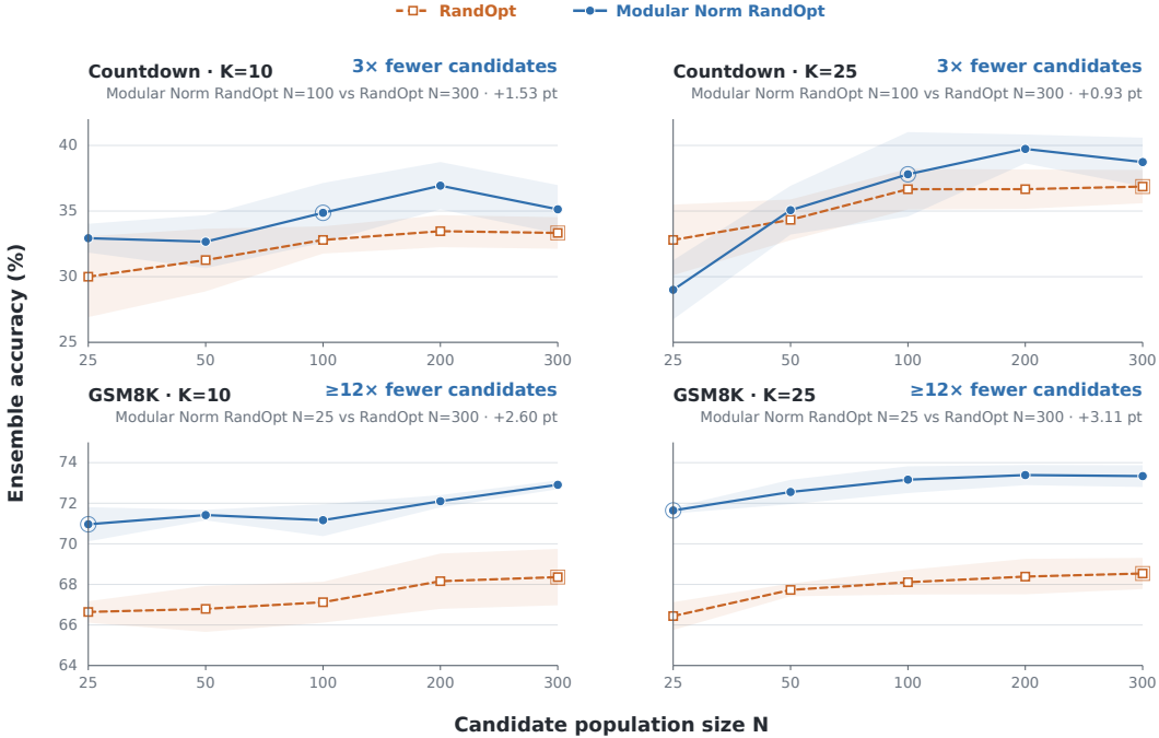
Figure 2: Population scaling on Countdown and GSM8K. At both K = 10 and K = 25 , Modular Norm RandOpt exceeds the N = 300 RandOpt reference using N = 100 candidates on Countdown and N = 25 on GSM8K. Curves show means and shaded regions show one sample standard deviation over seeds 42, 43, and 44. Population sizes are nested prefixes of the same N_{\max} = 300 population within each run.
