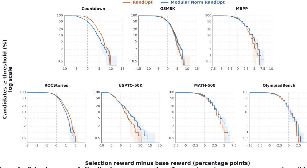
Figure 3: Selection-reward distributions across tasks. Curves show the mean percentage of candidates exceeding each selection-reward-gain threshold; shading shows mean \pm one sample SD across seeds 42–44, not confidence intervals. Bands are clipped to the displayed probability range.
