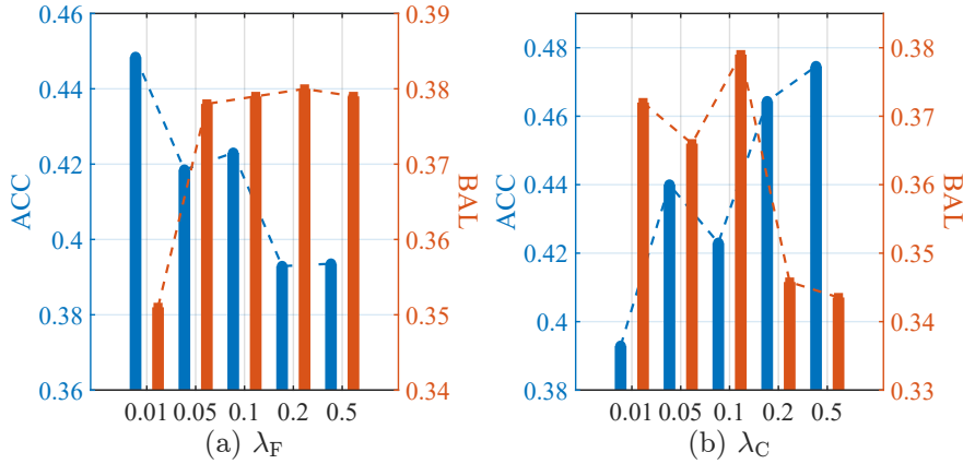
Figure 2: Parameter sensitivity analysis of \lambda_F and \lambda_C in terms of ACC and BAL.
