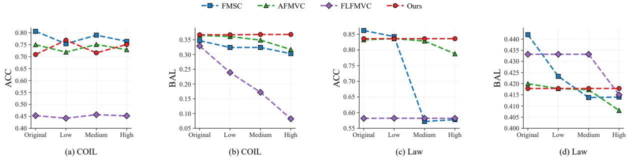
Figure 3: Comparison of multi-view fair clustering methods under increasing cross-view sensitive-information heterogeneity.
