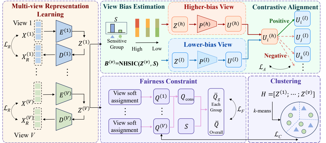
Figure 1: Overview of the proposed multi-view fair clustering framework.
