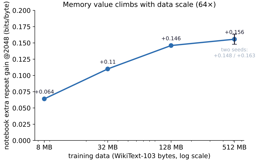
Figure 3: Notebook extra repeat gain at 8× training length vs training data (log axis). 64× data, 2.4× gain; two-seed error bar at the top rung.
