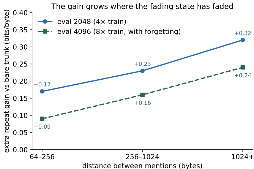
Figure 2: Extra repeat gain vs distance between mentions (WikiText-2 bytes). The notebook’s benefit grows exactly where the fading state has faded, and holds at 4× and 8× the training length.
