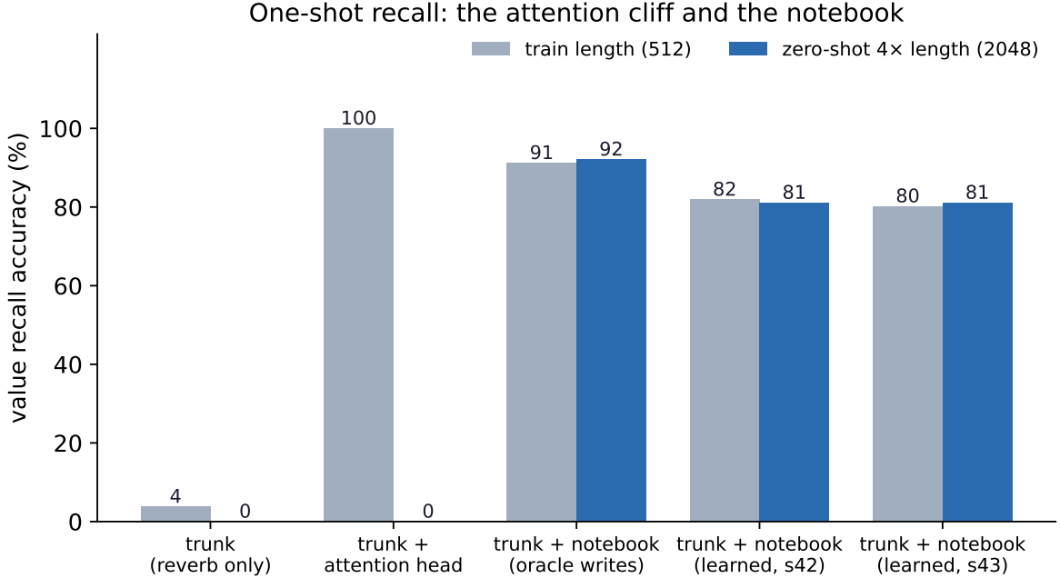
Figure 1: One-shot recall at training length (512) and zero-shot at 4 \times length (2048). The attention head is perfect inside its training length and zero beyond it; the notebook is length-invariant.
