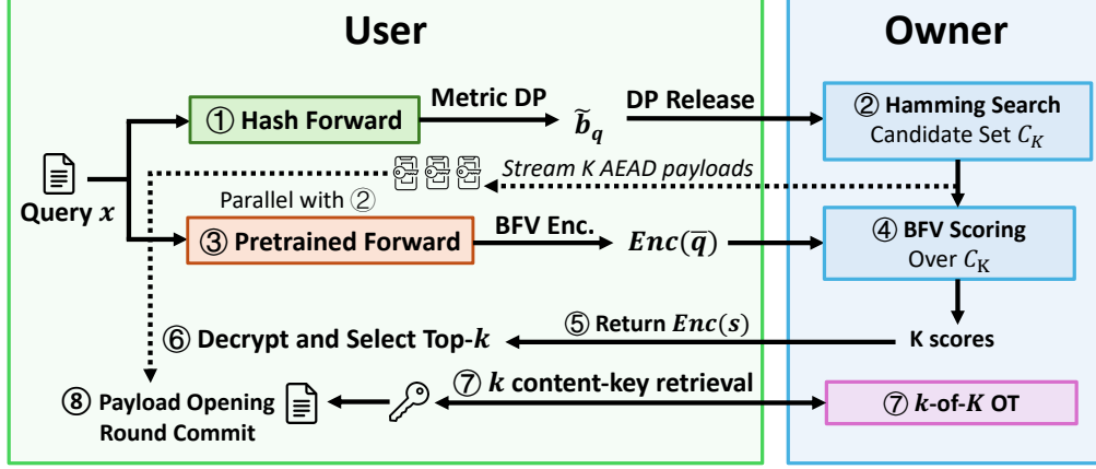
Figure 2: Online retrieval pipeline. Metric-DP Hamming shortlisting overlaps the pretrained scoring forward and query encryption. Once C_K is fixed, its AEAD ciphertexts stream during exact BFV scoring.
