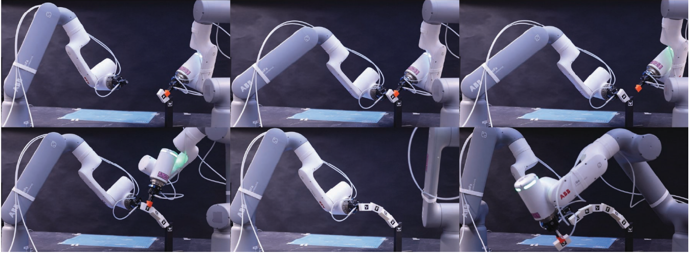
Fig. 11. Construction process using two robots. First row (left to right): the first robot places a block, the second robot supports it, and the first robot withdraws. After each placement, the camera captures the block positions, and our policy computes the next block’s target location. Second row: subsequent stages of the construction process.
