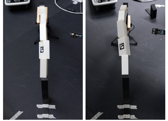
Fig. 10. Left: Structure built in closed-loop. Right: Structure built in open-loop. As one can see, the closed-loop is better aligned with the ground block.
