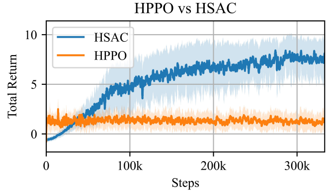
Fig. 6. Total reward accumulated during an episode. Results are averaged over three runs. As one can see, HPPO gets stuck in local minima and never reaches the maximum return.
