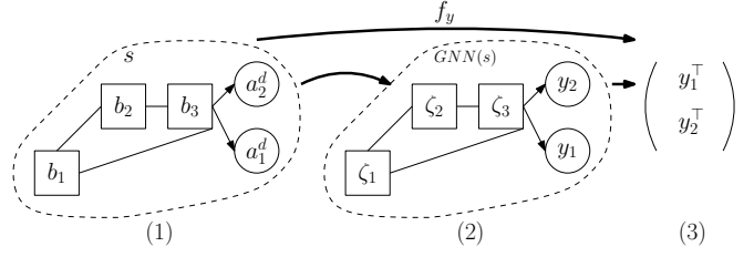
Fig. 4. GNN architecture. (1) Input state (the objective nodes are not drawn for simplicity) (2) Output of the GNN. The features attached to the block nodes \zeta can be seen as hidden states of a recurrent neural network and are discarded. (3) Output of the function f_y(s) , in this case, a matrix of size 2 \times n_y .
