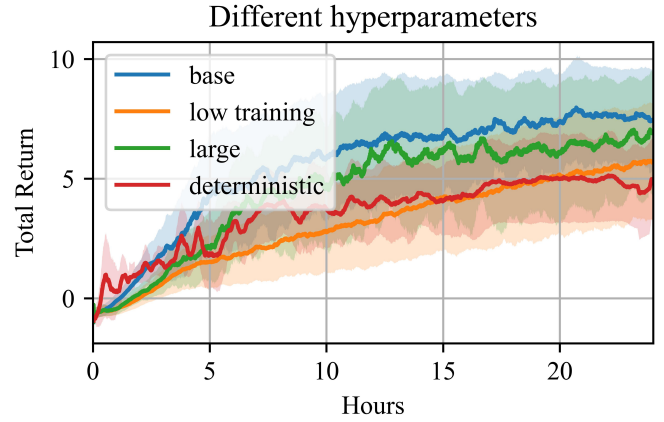
Fig. 7. Total reward accumulated during an episode. We used time rather than samples, as the duration of a single step could vary widely. Results are averaged over three runs.
