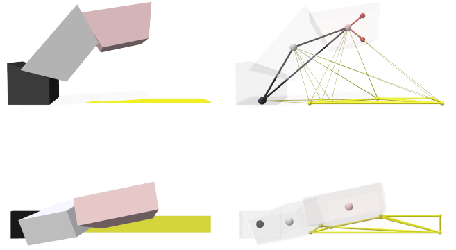
Fig. 2. Left: a simple three-block structure shown from two perspectives. The black block is the ground, the white block is free-standing, and the red block is held by a robot. Top right: the corresponding graph representation, showing block nodes \mathcal{N}_b , action nodes \mathcal{N}_a (red), and objective \mathcal{N}_o (yellow). Bottom right: detailed view of the objective subgraph, with corner nodes \mathcal{N}_o and the edges \mathcal{E}_{oo} connecting them in yellow.
