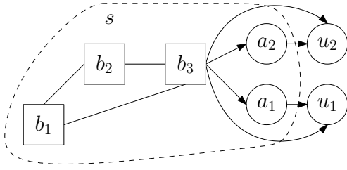
Fig. 5. The actions are attached to the state with unidirectional edges, ensuring that q_1 = q_1' in Equation 10. In this example, the state is composed of 3 blocks, and the two possible block types that can be added. The objective nodes are omitted for simplicity.
