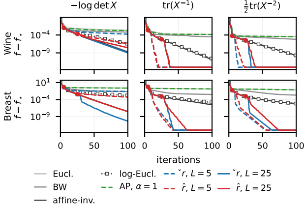
Fig. 1. Objective gap for (26) against iterations at \mu = 0.01 . Rows correspond to the two datasets, and columns to the three regularizers. The regularizers are labeled by R - \text{tr} X , as in Table 2. All runs start from X_0 = I and use the same line search. The two-stage curves run at the default r = 2 , the affine-invariant weight, until the marker at L and branch there. A five-step pilot suffices on the barriers but not under the log-determinant, which is why L = 25 is used throughout. Log-Euclidean carries open squares because it can sit under affine-invariant to within half a percent.
