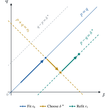
Fig. 3. Selecting the exponent and shape in the (p, q) family. Blue marks the first exponent fit on p = q . Yellow selects \delta^* along p + q = r_0 , and green refits the exponent along p - q = \delta^* . The gray branch contains the same metrics with p and q exchanged. The positions are schematic. The arrows give the selection order. The final fit can move in either direction along the green line.
