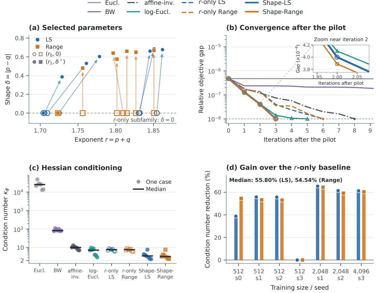
Fig. 4. Exponent and shape tuning on SARCOS over seven cases. (a) Open markers show (r_0, 0) and filled markers show (r_1, \delta^*) . (b) Median relative objective gap after the shared 25-iteration affine-invariant pilot. Completed runs are held at 10^{-8} for aggregation. The inset enlarges the second iteration after the pilot. (c) Condition number \kappa_\phi of the full preconditioned Hessian at X_{\text{ref}} . Each point is a case and black bars mark medians. (d) Percentage reduction 100(1 - \kappa_\phi / \kappa_{r_0}) relative to the corresponding r -only baseline. Each baseline uses the initial exponent r_0 from the same fitting rule with \delta = 0 .
