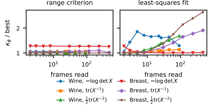
Fig. 2. Conditioning delivered against the number of frames read, over the six settings of (26) at \mu = 0.01 , with the range criterion (21) on the left and the least-squares fit (20) on the right. Curves are named by dataset and by R - \text{tr} X as in Table 2. Each value is \kappa_\phi at the exponent the criterion returns, divided by the best any diagonal member attains, so 1 is the floor of the sweep. Each subset contains the pair S_0 from Proposition 7. Additional frames are sampled at random. The curves show the median over twelve draws at each subset size. Reading more frames does nothing for the range criterion and hurts the least-squares fit.
