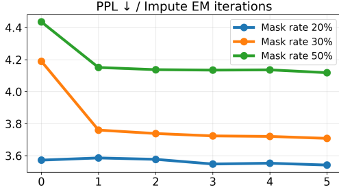
(b) PPL ↓ versus number of Impute-EM iterations across mask rates.
