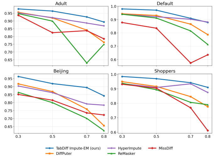
Fig. 2: Overall Density ↑ under MCAR versus missing rate (Adult, Shoppers, Default, and Beijing). Overall Density is (Trend + Shape)/2.
