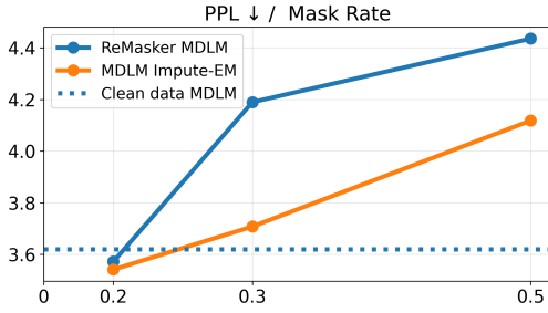
(a) PPL ↓ versus mask rate. ReMasker MDLM and Clean data MDLM as baselines, compared with MDLM Impute-EM (ours).
