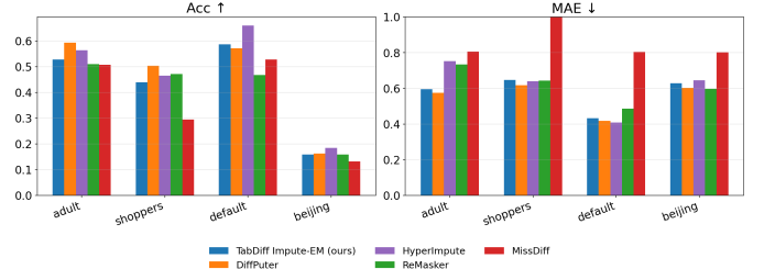
Fig. 8: Discriminative metrics under MNAR at mask rate p = 0.7 . Categorical accuracy \uparrow and MAE \downarrow across the four datasets.
