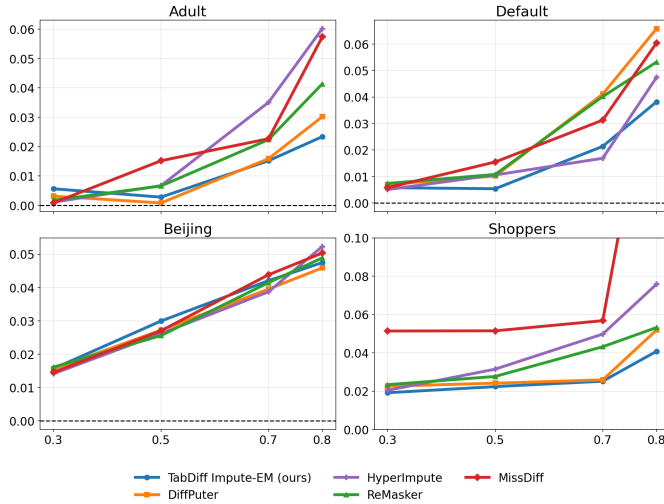
Fig. 3: ML-efficiency absolute deviation \downarrow under MCAR versus missing rate (Adult, Shoppers, Default, and Beijing), relative to the MLE on the clean dataset. Lower is better. Beijing MLE is multiplied by 0.1 to keep the scale comparable across datasets.
