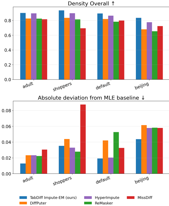
Fig. 4: Under MNAR at mask rate p = 0.7 : Overall Density \uparrow and ML-efficiency absolute deviation \downarrow across the four datasets. Beijing MLE is multiplied by 0.1 to keep the scale comparable across datasets.
