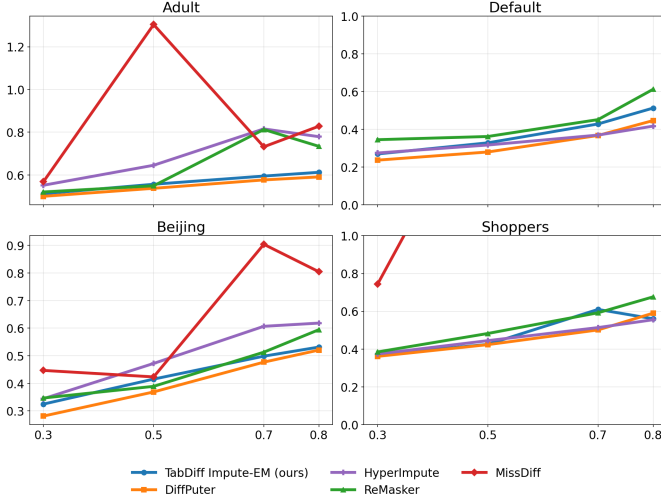
Fig. 7: Mean absolute error (MAE) \downarrow on numerical features under MCAR versus mask rate (Adult, Shoppers, Default, and Beijing).
