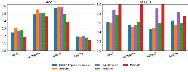
Fig. 10: Single-run MAR discriminative results under the DiffPuter 70% mask, split 0. Categorical accuracy \uparrow and MAE \downarrow across the four datasets. The MAE axis is capped at 1.0.
