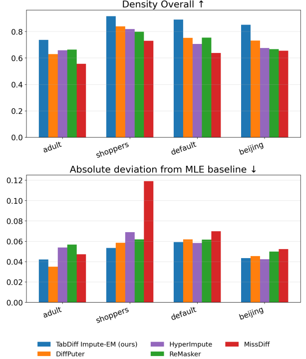
Fig. 9: Single-run MAR results under the DiffPutter 70% mask, split 0. Density Overall \uparrow and absolute deviation from the clean-data MLE baseline \downarrow across the four datasets. Beijing MLE deviation is multiplied by 0.1 to keep the scale comparable across datasets.
