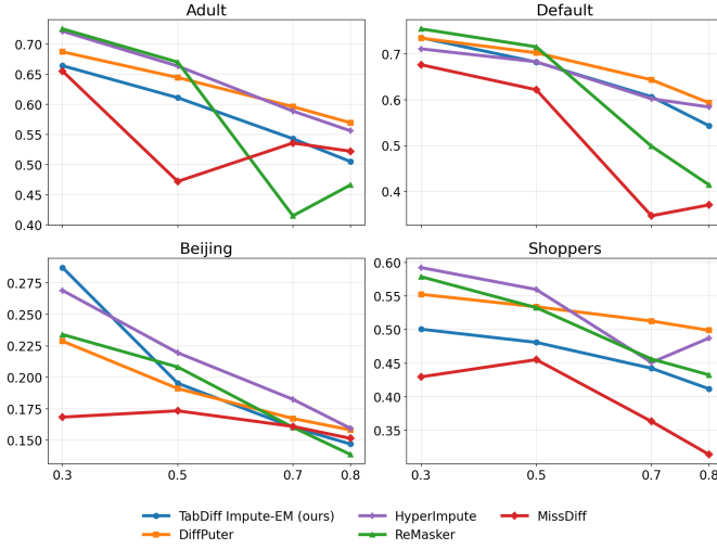
Fig. 6: Categorical accuracy \uparrow under MCAR versus mask rate (Adult, Shoppers, Default, and Beijing).
