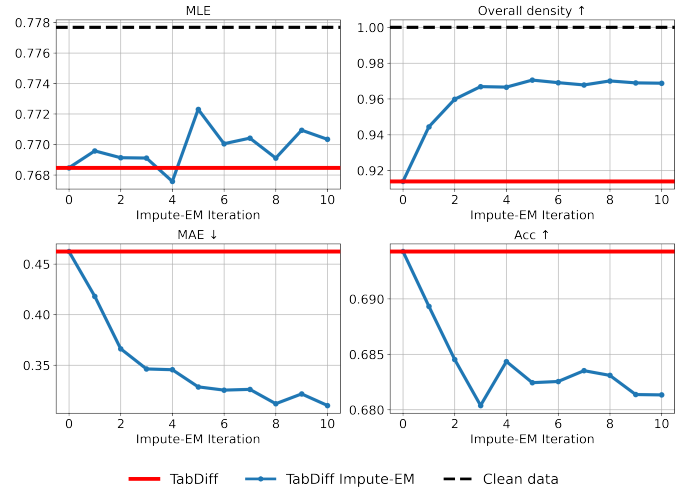
Fig. 5: Metrics versus Impute-EM iteration on the tabular data, i.e., "default" dataset with 50% missingness.
