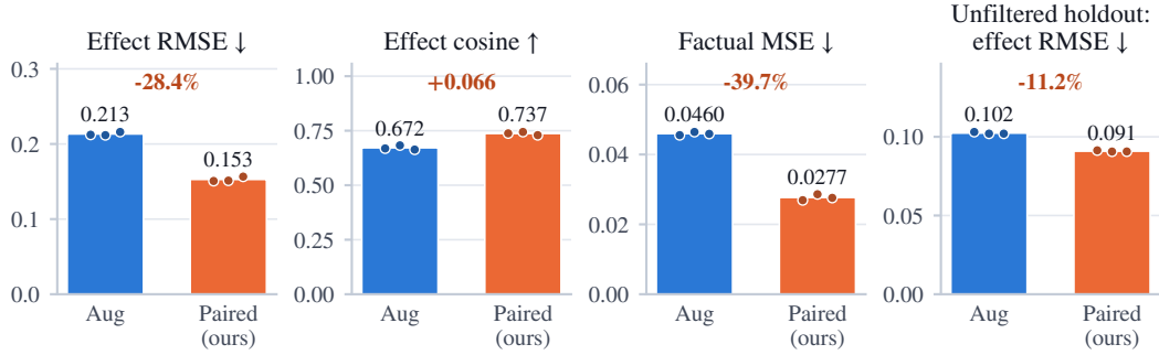
Figure 3: Effect loss on LeWM, pixel Push-T. AUG and PAIRED see the same paired images; PAIRED adds \mathcal{L}_{\Delta} . Latent metrics; means over three fresh seeds (dots: seeds); red: relative change (absolute for the cosine, taken over all pairs). Panels 1–3: held-out pairs from the training distribution (half responsive); panel 4: outcome-unfiltered holdout (6.5% responsive).
