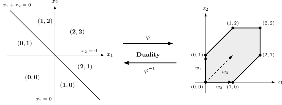
Figure 1: Illustration of the duality between zonotopes and bias-free two-layer ICNNs for W = (w_1, w_2, w_3)^\top with w_1 = (0, 1) , w_2 = (1, 0) , and w_3 = (1, 1) . The ICNN computes f: \mathbb{R}^2 \rightarrow \mathbb{R} , x \mapsto \sum_{i=1}^3 \max\{0, w_i^\top x\} (left) and the corresponding zonotope is Z(W^\top) = \sum_{i=1}^3 \text{conv}(\{0, w_i^\top x\}) (right). The hyperplanes w_i^\top x = 0 partition the input space into six linear regions. The gradient on a region is the sum of a subset of generators (bold vectors on the left) and is exactly one of the six vertices of Z(W^\top) .
