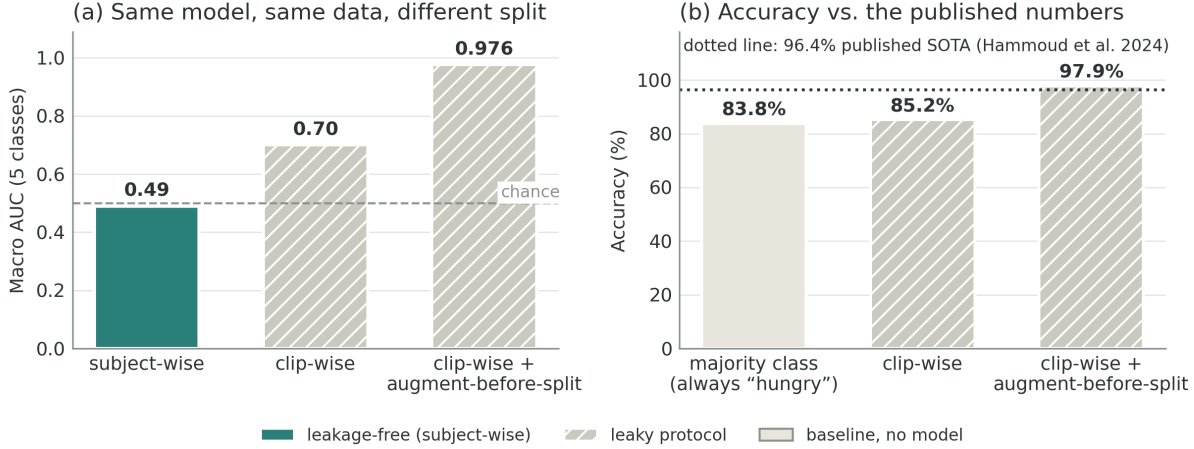
Figure 2: The leakage ladder on donatecry. Left: one model, one dataset, three split protocols; only the subject-wise protocol (solid) is valid. Right: the leaky protocols land on the accuracy range published as state of the art, and the majority-class baseline shows how little unbalanced accuracy means on this corpus.
