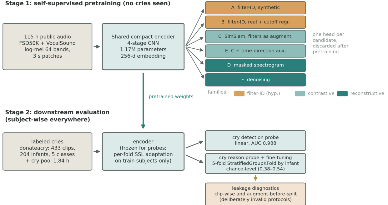
Figure 1: Study design. Stage 1: one compact encoder is pretrained six times, once per pretext task, on 115 hours of public audio that contains no infant cries; the task heads are discarded. Colors group the tasks into three families. Stage 2: the pretrained encoder is evaluated on labeled cries with subject-wise splits everywhere, including inside the per-fold SSL adaptation; the deliberately invalid protocols at the bottom exist only to measure leakage.
