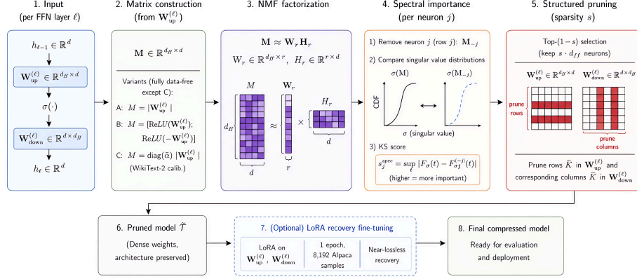
Figure 1: LILA framework. (1) For each FFN layer, a non-negative matrix M is constructed (2) from W using one of three variants, (3) factorized with rank- r NMF, and (4) each neuron j is scored by the Kolmogorov–Smirnov distance between the singular value distributions of M and the neuron-ablated matrix M_{-j} . (5) The lowest-scoring (1 - s) fraction of neurons are pruned by removing rows in W and corresponding columns in W^{(e)} . (6) The resulting pruned LLM preserves the dense architecture and can be optionally fine-tuned with LoRA for recovery.
