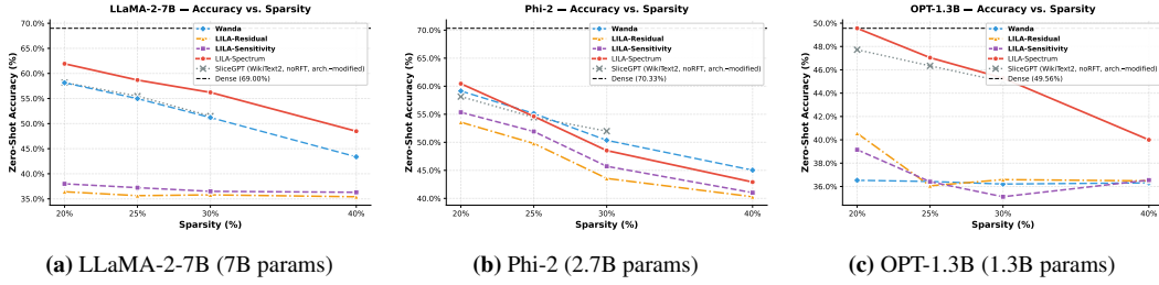
Figure 2: Zero-shot accuracy (%) vs. sparsity. All curves are zero fine-tuning (noRFT), WikiText-2 evaluation. LILA-Spectrum ( solid red ), LILA-Sensitivity ( purple dashed ), LILA-Residual ( orange dash-dot ): calibration-free, arch.-preserving. Wanda ( blue ): 128 WikiText-2 calibration samples, arch.-preserving. SliceGPT ( grey dotted ): 1,024 WikiText-2 samples, arch. permanently modified ; from Table 7 of Ashkboos et al. [2024]. LILA-Spectrum (data-free) outperforms SliceGPT (WikiText-2 calibrated) by +5.2–6.0 pp across all settings without accessing any data. Dense: black dashed baseline.
