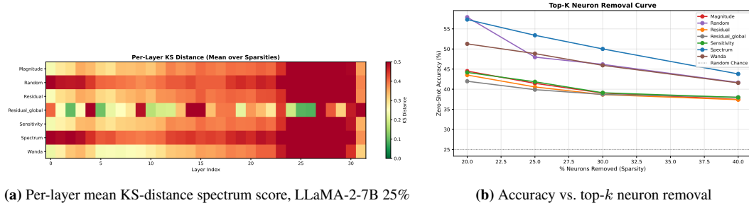
Figure 4: Layer-wise spectral analysis. (a) Early (0–5) and final (28–31) layers exhibit systematically higher KS-distance scores, indicating greater spectral sensitivity to neuron removal. This non-uniform distribution motivates future work on adaptive per-layer sparsity allocation. (b) Accuracy degrades sharply when the highest-scored neurons are removed (top- k curves), confirming that the KS-distance score correctly identifies functionally critical neurons.
