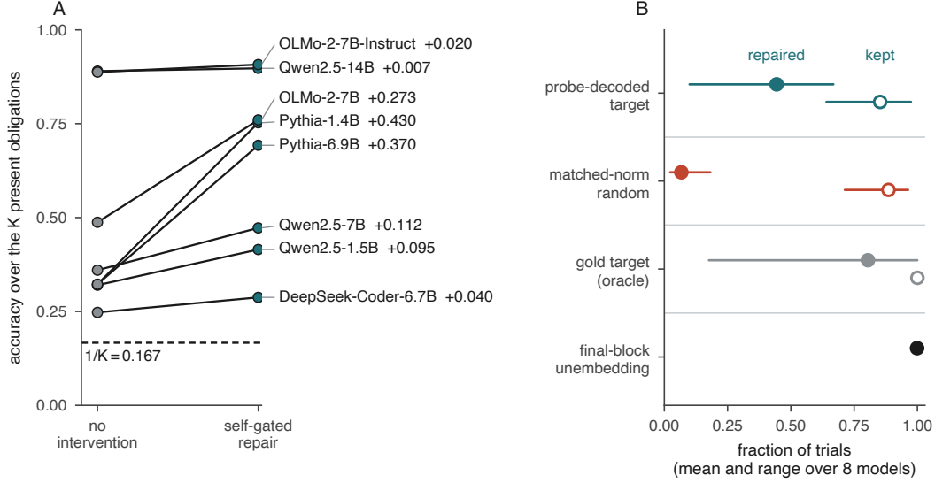
Figure 3: Self-gated activation repair raises accuracy on all eight models. (A) Accuracy without intervention and under the self-gated repair, one line per model, at \alpha = 0.5 on 1200 trials with K = 6 and D = 256 . The decoded arm uses no gold label and the direction is zero when probe and output agree. The dashed line is 1/K = 0.167 . (B) Control arms over the same eight models. Filled markers, labelled “repaired”, give the fraction of wrong trials an arm repairs; open markers, labelled “kept”, give the fraction of correct trials it preserves. Each is a mean with the range across models. The gold-target arm bounds what the read layer can do when the target is correct; the final-block unembedding arm checks the wiring and is measured on wrong trials only.
