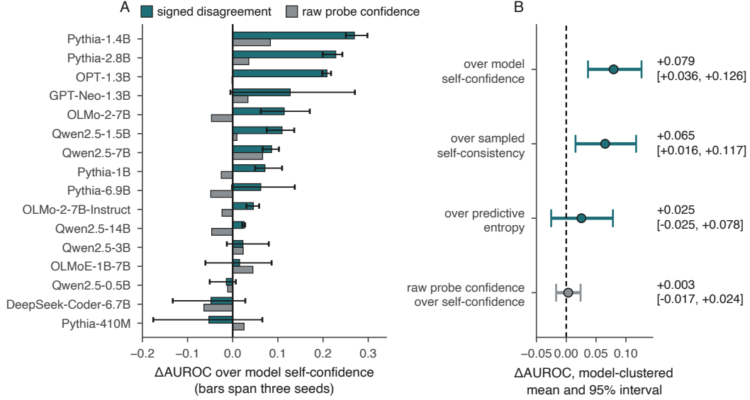
Figure 2: Signed disagreement improves failure detection over self-confidence. (A) Per-model change in AUROC relative to self-confidence, for the signed disagreement score and for raw probe confidence, on the same test trials with the same probe. Bars span three seeds. (B) Aggregate comparisons against four reference detectors, each a mean over 16 models with a 95% interval from a bootstrap clustered on model. The interval against predictive entropy crosses zero, and so does the interval for raw probe confidence against self-confidence.
