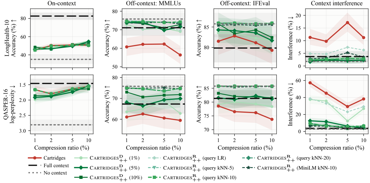
Figure 24 Gemma-4-E4B-it mitigation variants at 1-10% compression factor. Cartridges, 1/5/10% Dolci mixtures, and five router variants, using the rows and metrics of Figure 20. Shading shows available 95% intervals.
