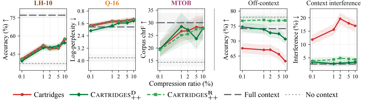
Figure 6 CARTRIDGES_{++}^D ( C_{++}^D ) and CARTRIDGES_{++}^R ( C_{++}^R ) across compression factors. Cartridges, C_{++}^D 5%, C_{++}^R kNN-10 on Qwen3-4B-Instruct-2507. Left: on-context metrics. Right: off-context accuracy and interference averaged over all three datasets.
