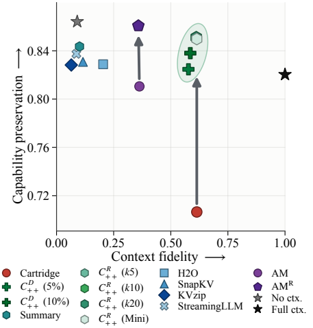
Figure 7 CARTRIDGES_{++} results on Gemma-4-E4B-it. LH-10/Q-16 across 1–10% compression (composite defined in Appendix E.1).
