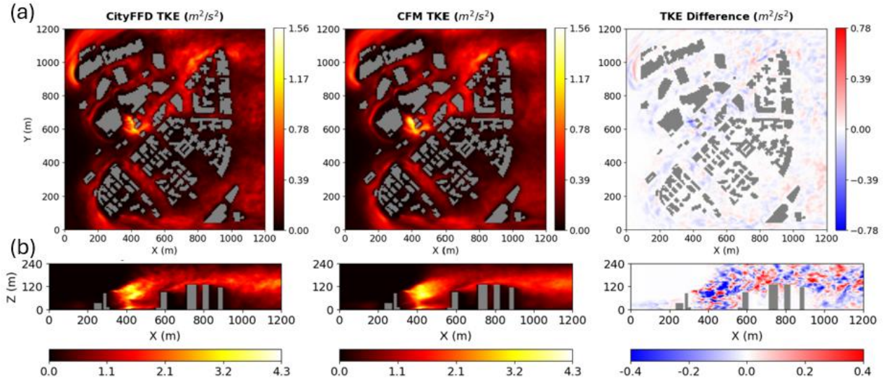
Figure 11: TKE maps. Left: CityFFD (35 snapshots); Center: CFM (35 snapshots); Right: difference. for (a) z=3 and (b) central yz plane
