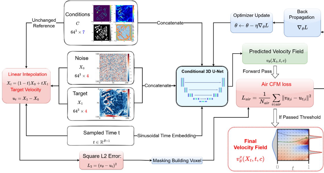
Figure 3: CFM training and generation pipeline. Left: conditioning inputs concatenated with noisy state; center: U-Net predicts velocity field V_{\theta} ; right: training target and generation.
