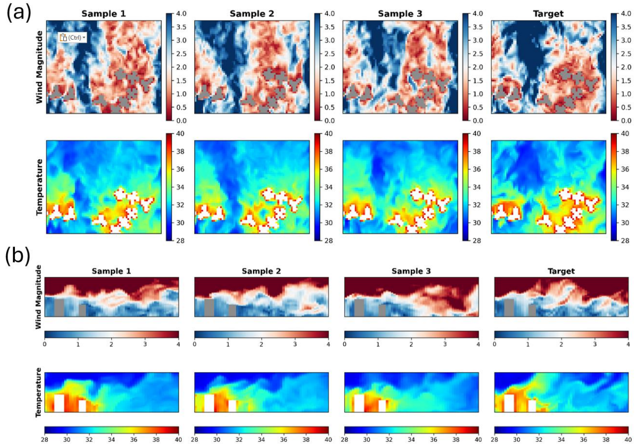
Figure 8: Zoomed-in Visual comparison of wake region: generated snapshots samples (first 3 columns) vs. random CityFFD reference snapshot (right column) at (a) horizontal slice of z = 135 m and (b) xz vertical plane in the center
