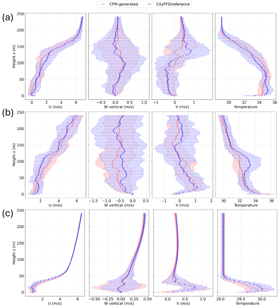
Figure 13: Multi-site vertical profiles for u , w , v , T at (a) open area, (b) city canyon, and (c) upstream locations (last row). Solid lines: ensemble mean; horizontal bars: variable range at each height for ensemble.
