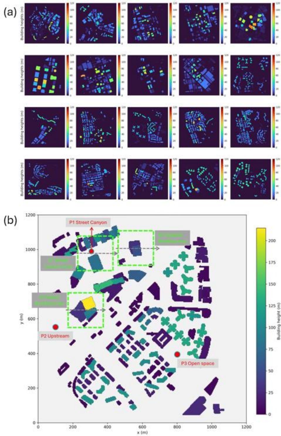
Figure 2 (a) Urban morphology of all cases in the dataset colored with height (b) Urban morphology of the testing case and focused areas for validation
