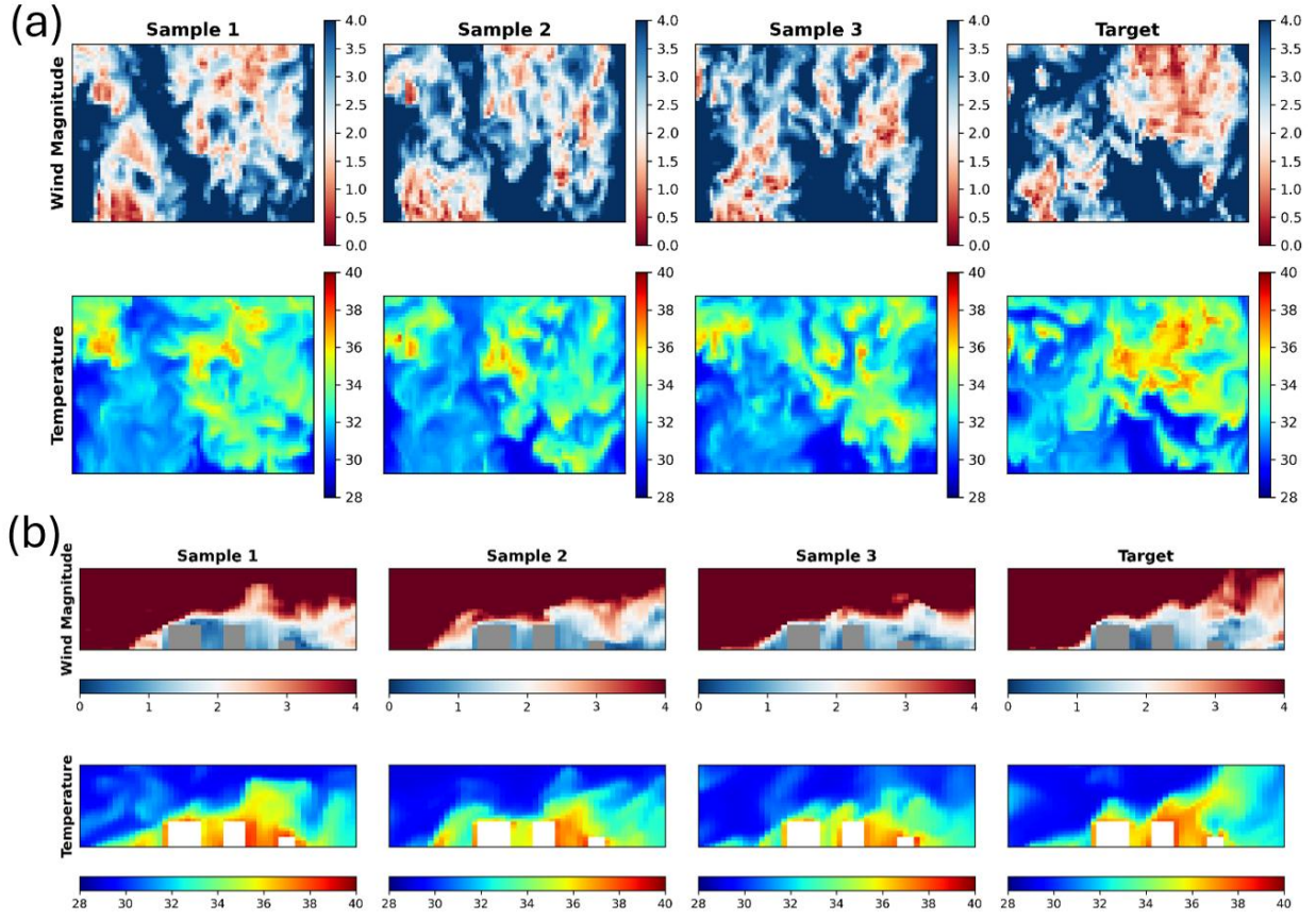
Figure 7: Zoomed-in Visual comparison of above-roof region: generated snapshots samples (first 3 columns) vs. random CityFFD reference snapshot (right column) at (a) horizontal slice of z = 100 m and (b) xz vertical plane in the center
