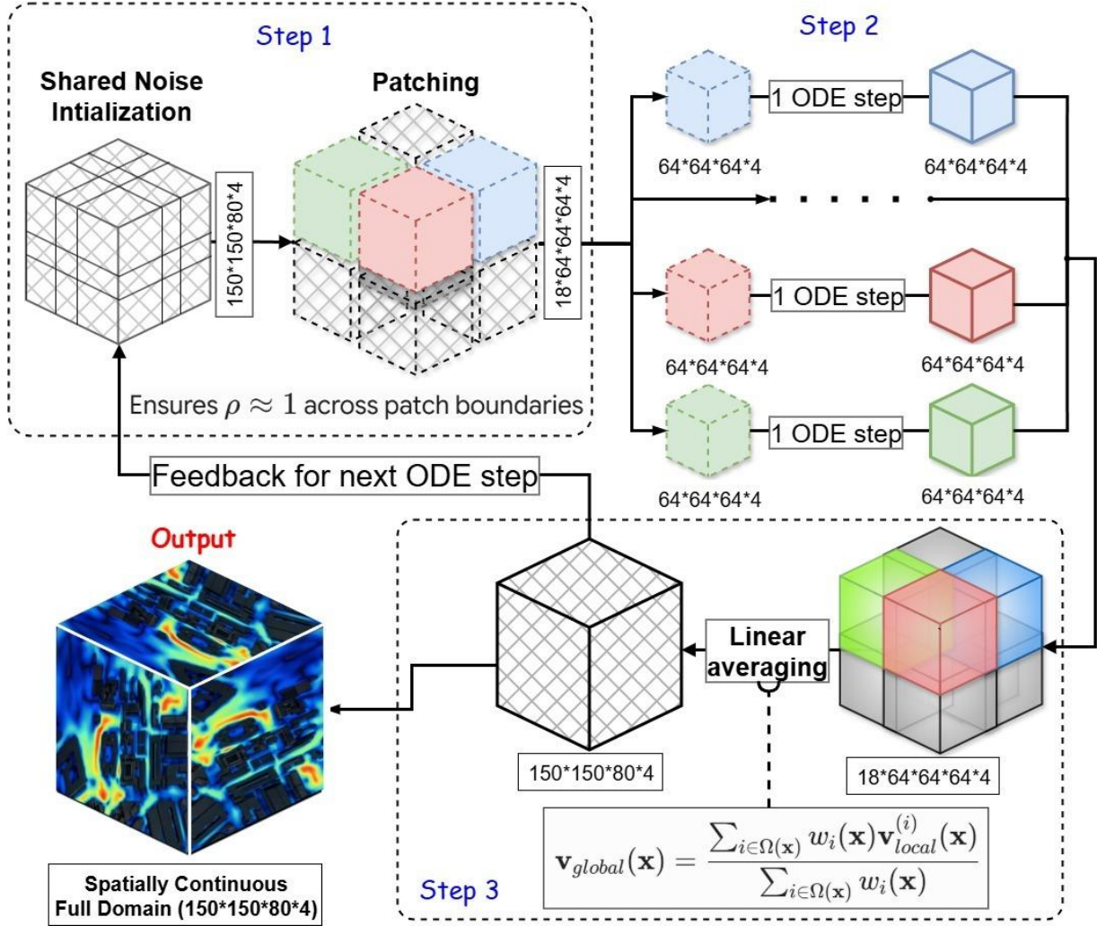
Figure 4 Schematic of the patch-based domain reconstruction: (a) overlapping 64^3 patches tiling the full domain; (b) shared-noise initialization; (c) per-step linear weighted averaging producing the full-domain field.
