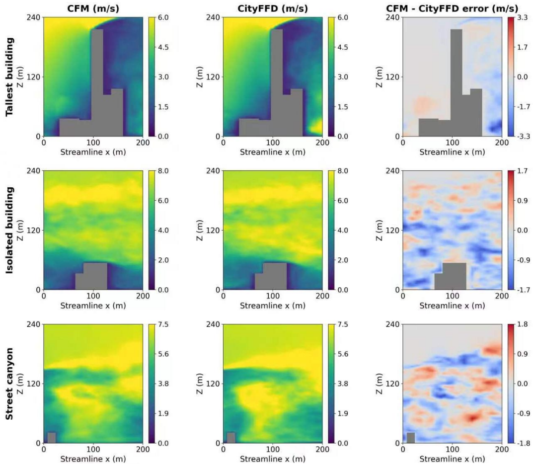
Figure 14: Wind gusts in vertical planes for regions of tallest building (top), isolated building (middle), and street canyon (bottom) from CFM, CityFFD and their error
