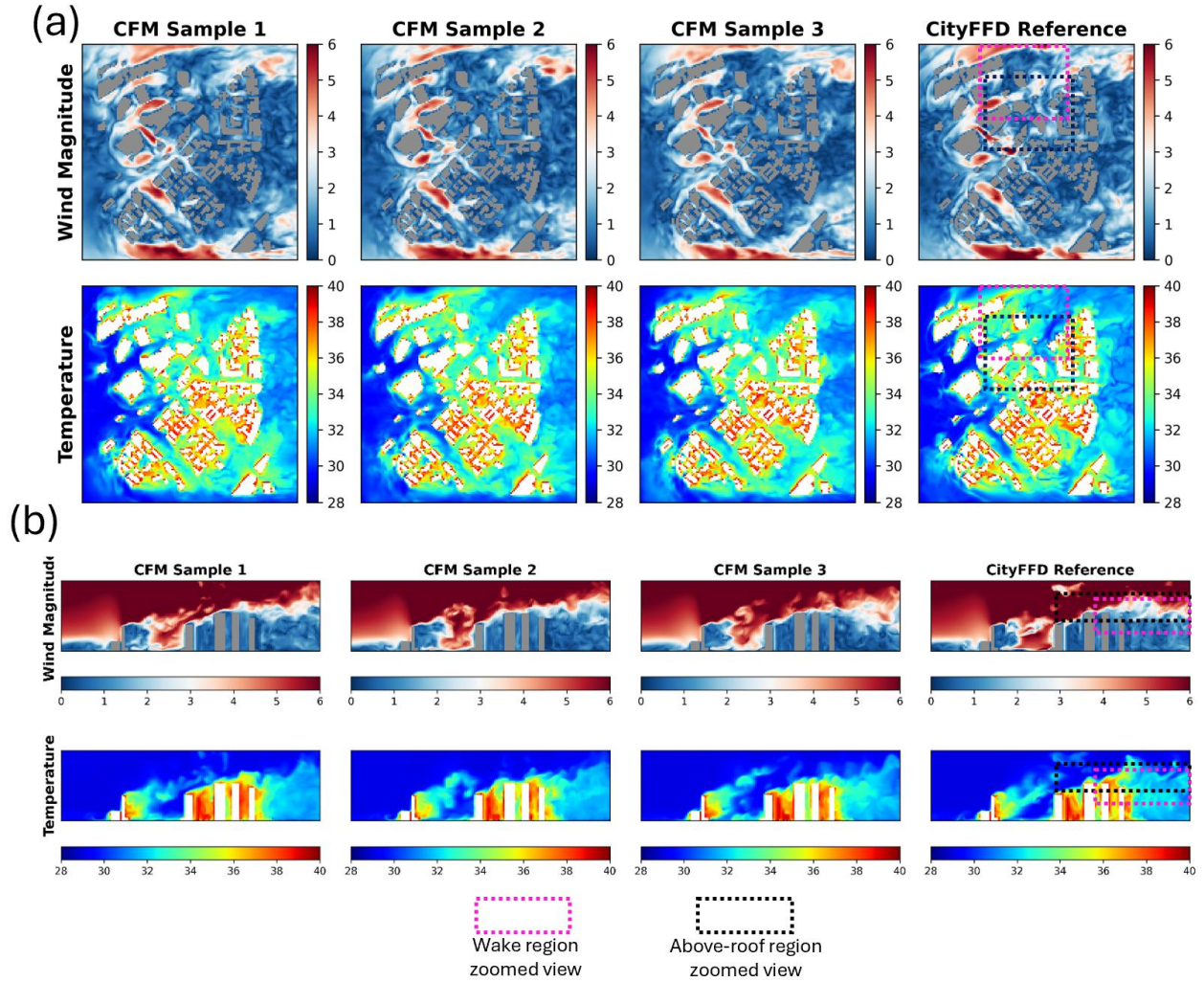
Figure 6: Visual comparison of generated snapshots samples (first 3 columns) vs. random CityFFD reference snapshot (right column) at (a) horizontal z = 3 m and (b) xz vertical plane in the center
