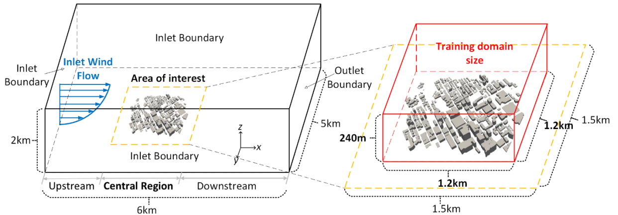
Figure 1 Computational Domain for CityFFD simulation (left) and target area for model training (right)
