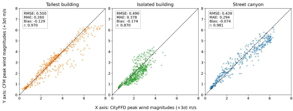
Figure 16: Parity plot of CFM predicted and CFD-simulated local 3\sigma peak wind speeds across 3 different urban configurations (Tallest building, Isolated building, and Street canyon)
