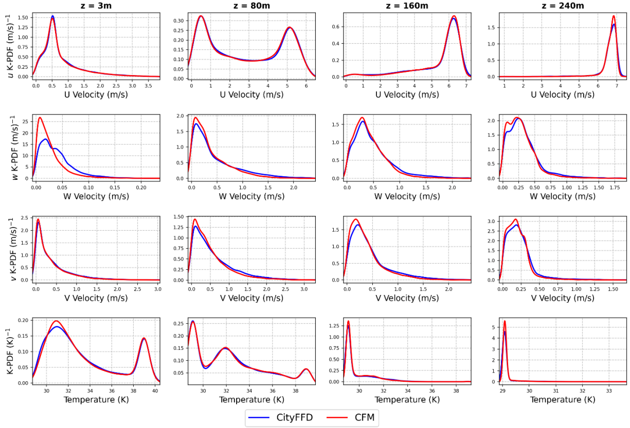
Figure 12: Kernel-PDF for u , w , v , T at multiple heights. Red: CFM (35 snapshots); blue: CityFFD reference (35 snapshots) for z=3\text{m} , 80\text{ m} , 160\text{ m} , and 240\text{ m}
