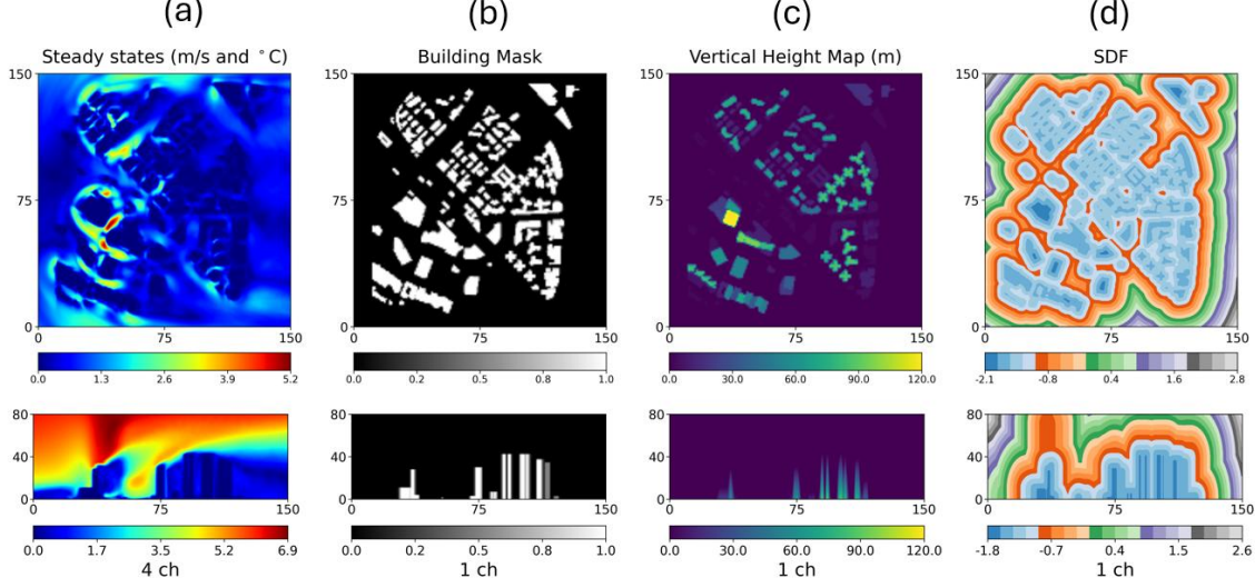
Figure 4: All Conditional inputs: (a)Time-Averaged Mean Flow Field; (b) Building Binary Masks and (c)Building Roof Height in meters and (d) Signed Distance Function of the Buildings
