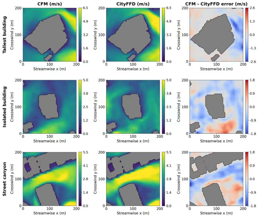
Figure 15: Wind gusts in horizontal planes ( z = 3\text{m} ) for regions of tallest building (top), isolated building (middle), and street canyon (bottom) from CFM, CityFFD and their error
