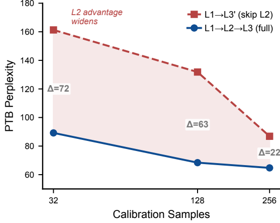
Figure 3: PTB test perplexity vs. calibration budget (LLaMA-7B, \rho=0.6 ). L2’s OOD advantage grows from \Delta=22 at 256 samples to \Delta=72 at 32 samples.
