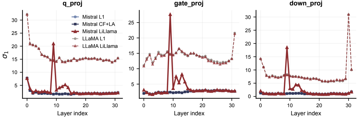
Figure 5: Leading singular value \sigma_1 of compressed weights by layer ( \rho=0.6 ). LiLlama (red, solid) amplifies Mistral-7B MLP \sigma_1 by 40–95% vs. L1 baseline (light blue). Our CF+LA (dark blue) preserves the baseline spectral structure. LLaMA-7B (dashed) shows milder amplification.
