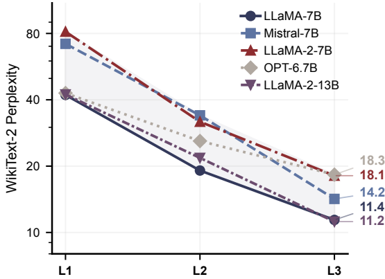
Figure 6: WikiText-2 test perplexity across optimization levels (L1→L2→L3) for five models (7B–13B) at \rho=0.6 . The chain generalizes across architectures, though per-level gains are model-dependent.
