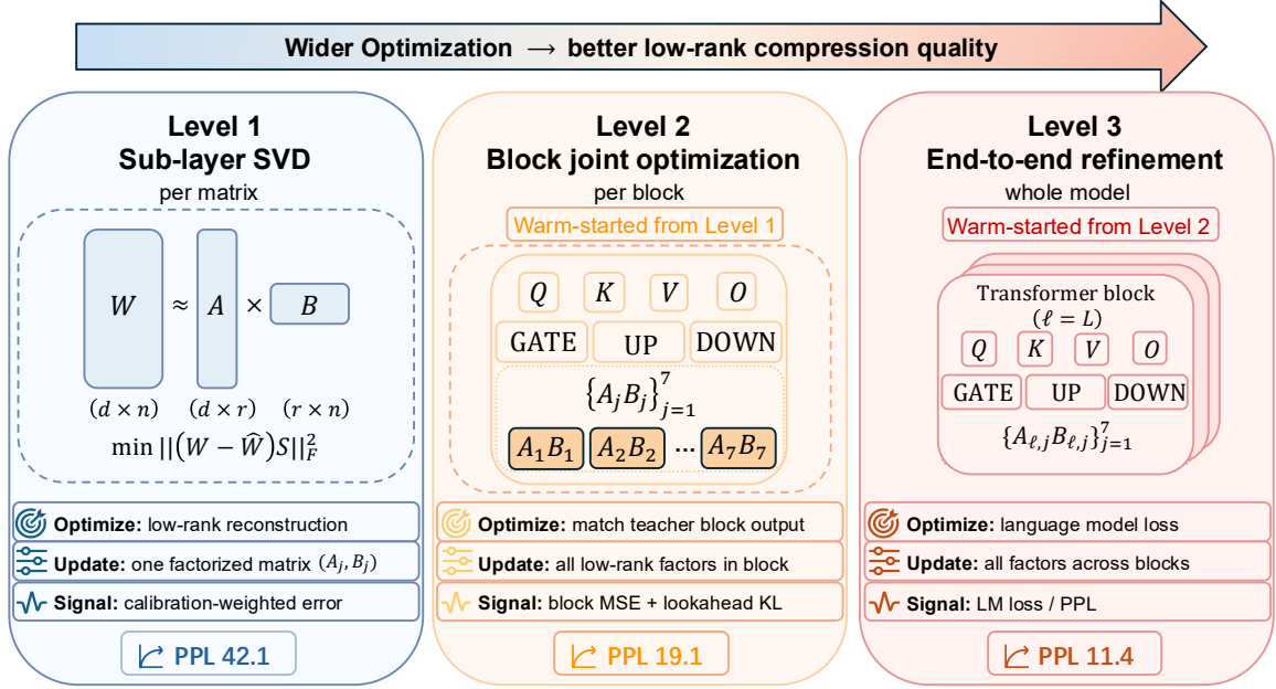
Figure 1: Three-level compression chain. Each level widens the optimization scope and warm-starts from the previous solution using the same calibration budget. Numbers: LLaMA-7B WikiText-2 PPL at \rho=0.6 . Each level reduces perplexity by roughly 2\times .
