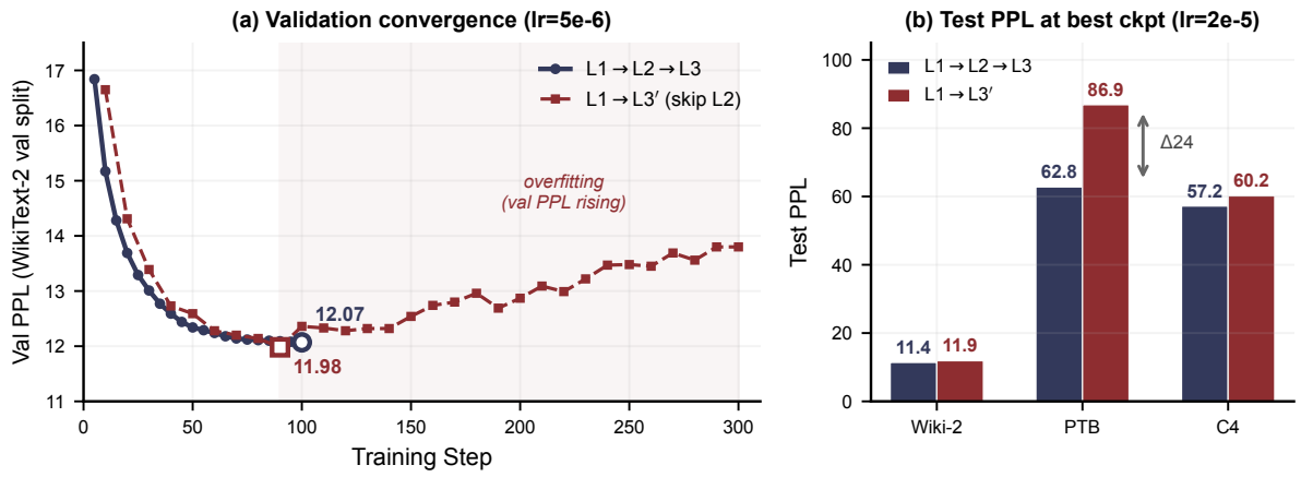
Figure 7: Skip-L2 ablation on LLaMA-7B at \rho=0.6 . (a) Validation PPL ( \text{lr } 5 \times 10^{-6} ) converges similarly, but skip-L2 overfits past step 90. (b) Test PPL at best checkpoint ( \text{lr } 2 \times 10^{-5} ): in-distribution (WikiText-2) matches, but OOD (PTB) diverges by 24 points.
