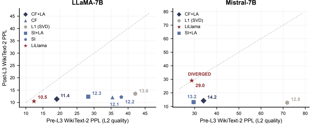
Figure 4: Pre-L3 vs. post-L3 WikiText-2 test perplexity ( \rho=0.6 , 256 calibration samples, best val checkpoint). Left: LLaMA-7B—better L2 warm-start yields better L3 (monotonic). Right: Mistral-7B—LiLlama achieves the best L2 but diverges at L3, coinciding with the spectral amplification of Figure 5.
