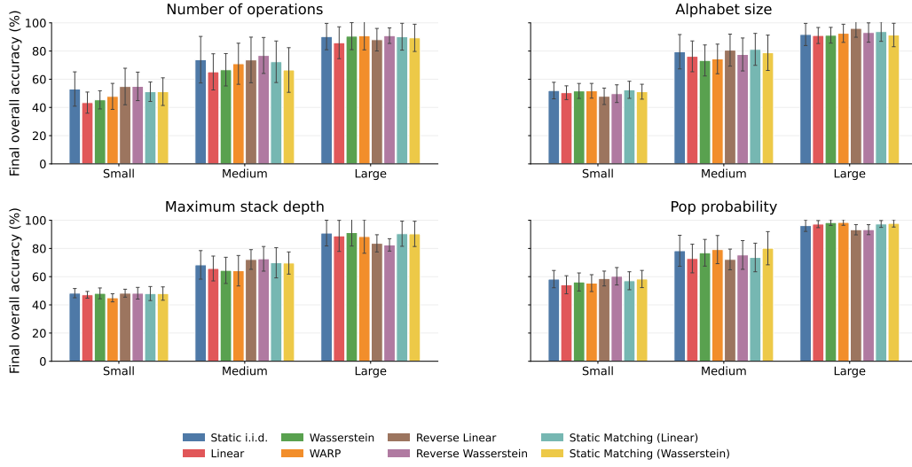
Figure 20: Task-wise final overall accuracy for Stack Operations. Panel titles denote the difficulty axes. Bars show mean final overall accuracy over 10 random-seed repetitions, and error bars show one standard deviation.
