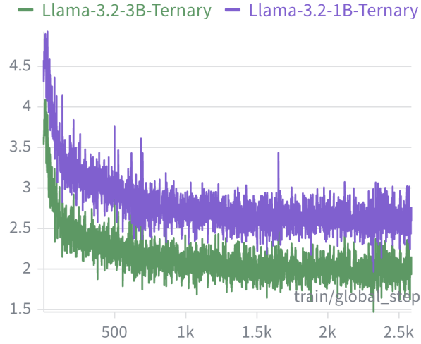
Fig. 2: Training loss on Llama-3.2-1B.
