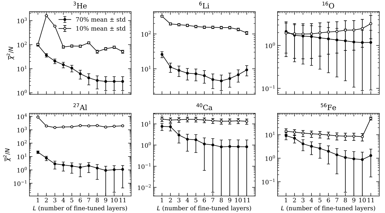
FIG. 5. Ensemble-averaged \bar{\chi}^2/N as a function of the number of fine-tuned layers, analogous to Fig. 4. The error bars denote the standard deviation across the 50 ensemble members.
