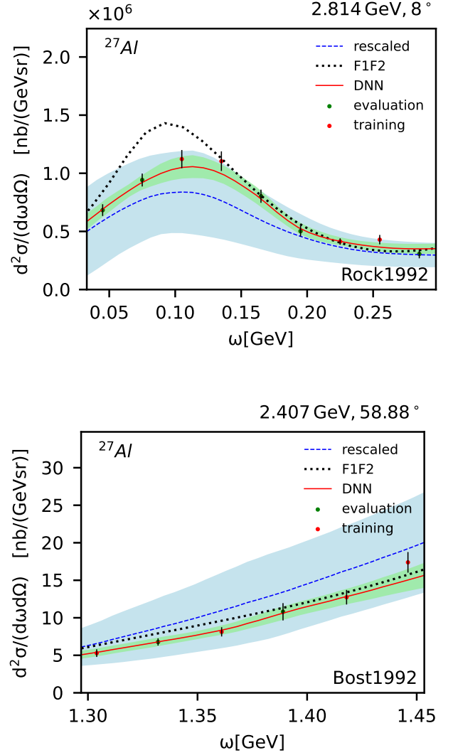
FIG. 14. Case (C): aluminum cross sections predicted by 70% training split model with 9 layers tuned. Electron energies 2.814 GeV (top) and 2.407 GeV (bottom) and corresponding scattering angles \theta = 8^\circ (top) and \theta = 58.88^\circ (bottom), respectively. The corresponding kinematics is illustrated in Fig. 13.
