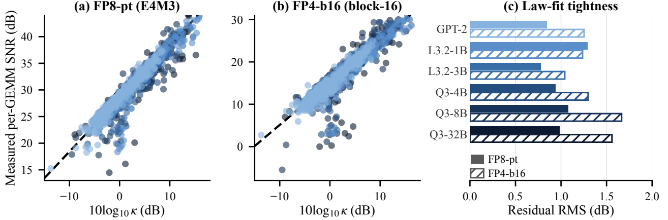
Figure 1. The noise law per GEMM cell. (a) Per-tensor E4M3 and (b) block-16 E2M1: measured SNR against 10 \log_{10} \kappa across the six families of Table 5. The dashed line is Eq. 8 at unit slope per decade with the intercept at the measured median C_{\text{fmt}} ; for E4M3 that median lies within 0.1 dB of the parameter-free prediction of §2.2. (c) RMS of the residual r (Eq. 9) per family and format, the statistic in which the shared numerator \mathbb{E}[S^2] cancels.
