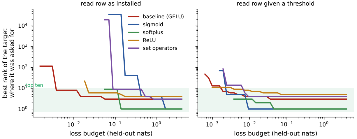
Figure 26: The best rank the target reaches for a given held-out loss budget, at layer ten. Each frontier is taken over four compensation arms and five write strengths. Left: the read row as installed. Right: the same with a threshold subtracted from the read row, swept over three quantiles.
