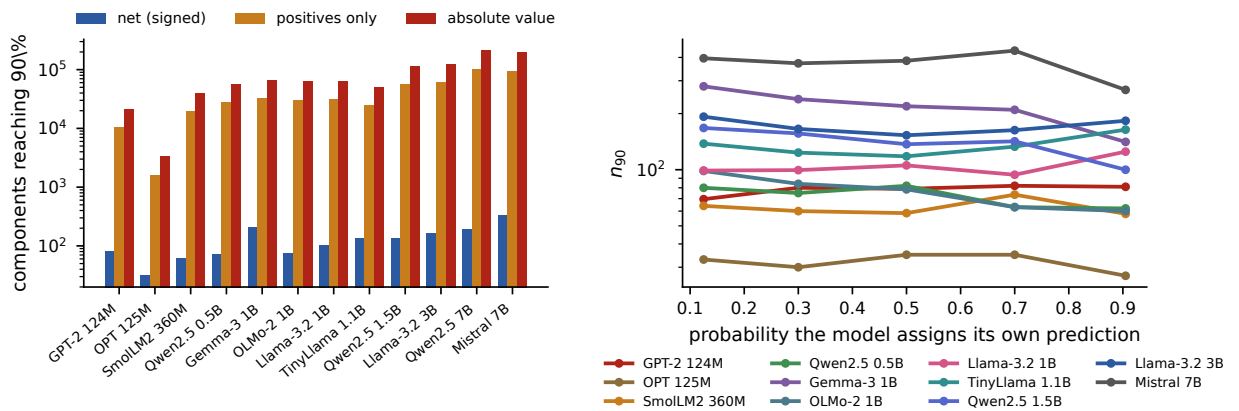
Figure 30: Left: the three denominators across the twelve models, on a log axis. The gap between the signed convention and the others is two to three orders of magnitude in every one. Right: circuit size against the confidence of the prediction, which is why all figures here are read at one floor.
