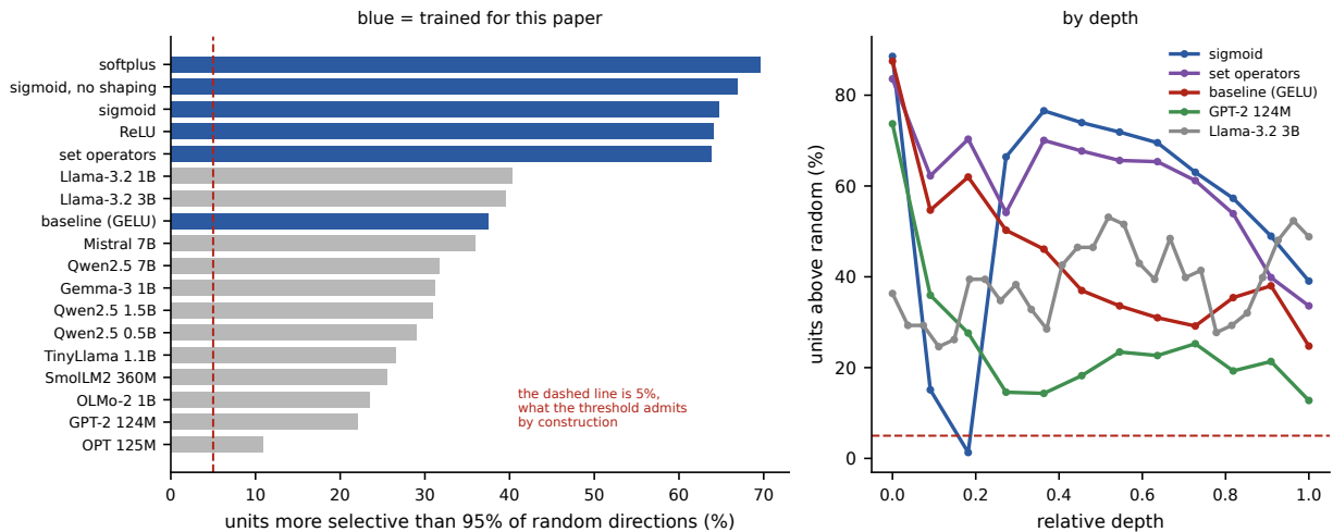
Figure 33: Left: the share of feed-forward units whose response to candidate tokens is more concentrated than 95 percent of random directions in the same layer. The dashed line is the 5 percent such a threshold admits by construction, so it is the level a model with no token-selective units would show. Right: the same quantity against relative depth. The constructions trained here hold their level through the body of the network, and the conventional baseline declines with depth.
