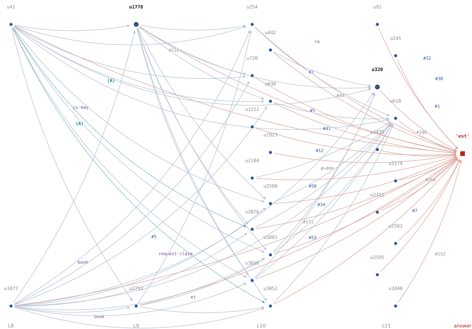
Figure 81: sigmoid, no shaping, prediction 4: the graph, 26 members and 47 edges among them.
