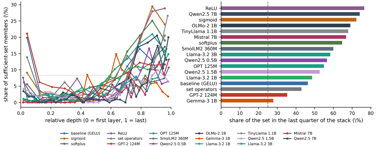
Figure 31: Where the sufficient circuits sit, across every model the search was run on. Left: share of the set’s members by relative depth, one line per model; the dotted line is what an even spread would give. Right: the share falling in the last quarter of the stack, against the 25 percent an even spread would put there. Members are those of the pruned sufficient sets of Section 2.5, not of the one-hop accounting.
