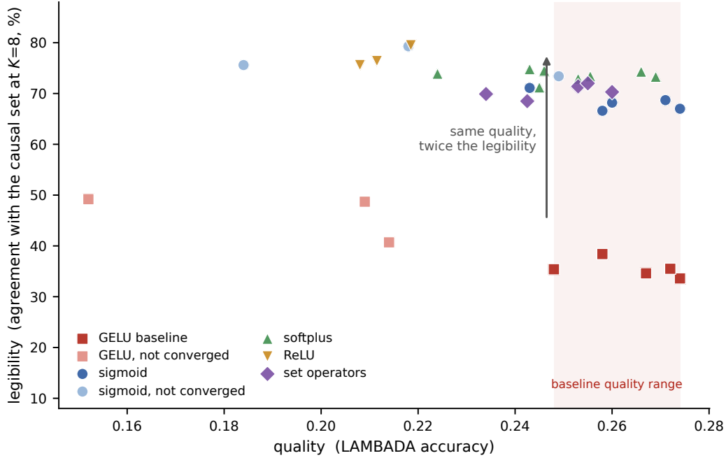
Figure 21: Every trained model in this paper. Horizontal axis is quality; vertical axis is how well a unit’s parameters name the tokens that causally drive it in the vocabulary basis , both under one protocol. Read in a different basis, the same units order their drivers well above chance (Section 3.4); what this axis measures is whether the token table is the right place to look, not whether anything is there. The shaded band is the baseline’s converged quality range. The baseline sits low and to the right — good quality, poor legibility — and every order-preserving arm sits about twice as high at the same quality; ReLU sits higher still and to the left, buying legibility with accuracy. In both families the pale points, the seeds that failed the convergence screen, sit above their own converged siblings without exception, which is why quality is on this axis at all.
