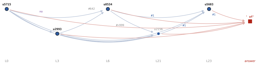
Figure 70: Qwen2.5 1.5B, predictions 1 and 2. Of 19 predictions drawn at random, these are two of the four whose sufficient set is nearest the median, 6.
