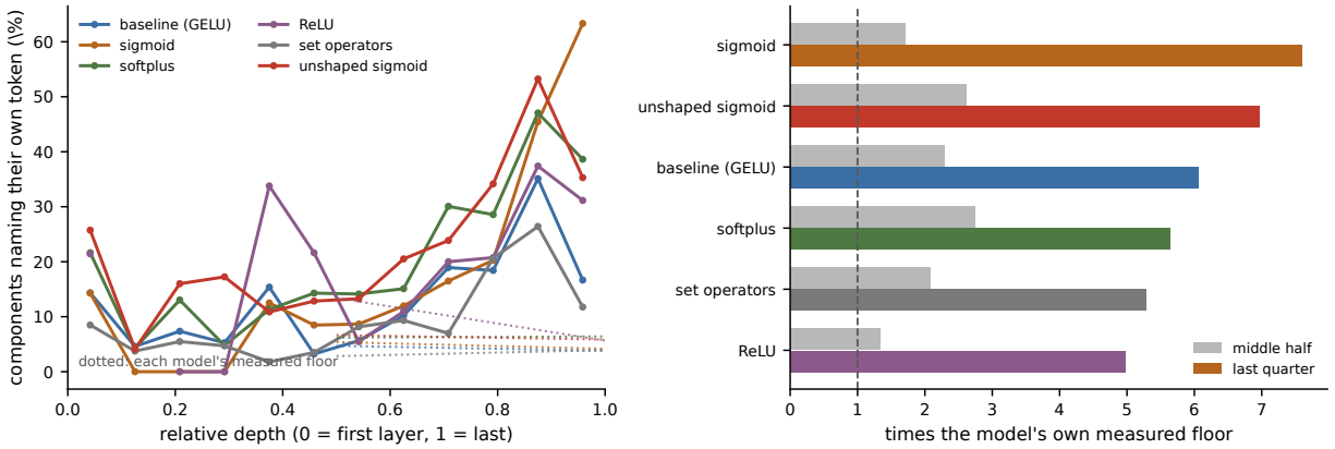
Figure 6: A component names its own token when the token the model predicts lands inside the top hundred of its write column's ordering over the vocabulary, signed by how the component fired. Left: the share by relative depth, one line per model, with each model's own measured floor dotted. Right: the middle half of the stack and the last quarter, as multiples of that floor, which is the only form in which models can be set beside one another. Rank exists only for components appearing in a trace, so this is conditioned on a component mattering to some prediction.
