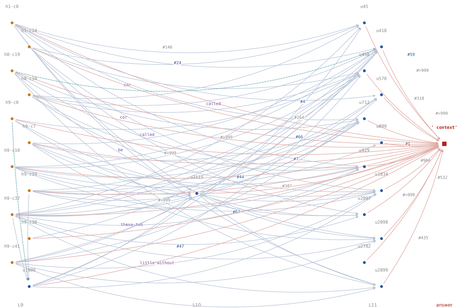
Figure 87: ReLU, prediction 4: the graph, 25 members and 70 edges among them.
