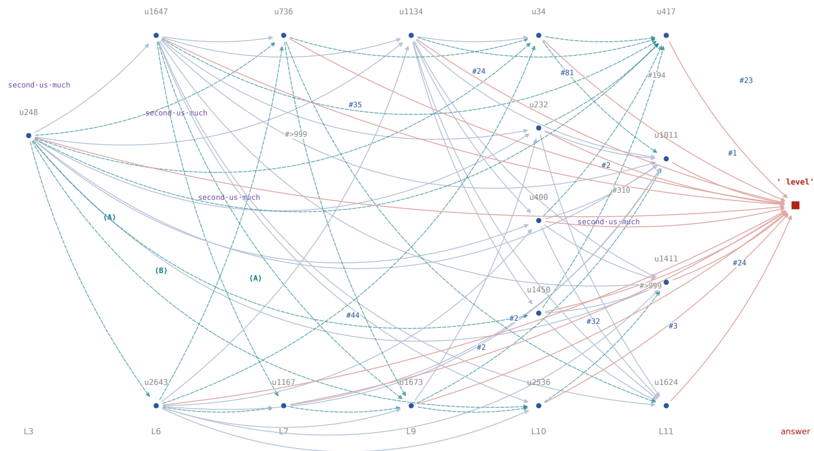
Figure 75: OPT 125M, prediction 3: the graph, 16 members and 59 edges among them.
