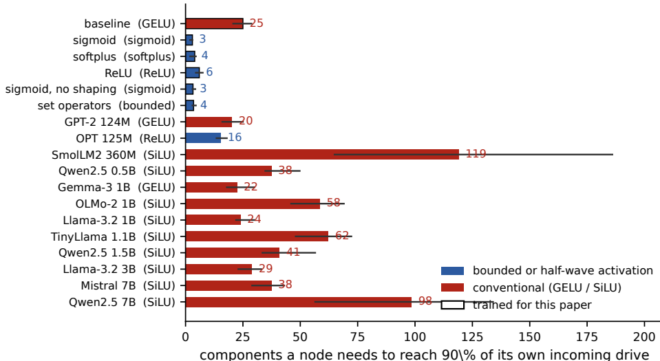
Figure 32: Branching factor with bootstrap intervals, every model in this paper. Outlined bars are the models trained here, which differ from one another only in the feed-forward unit; the rest hold nothing fixed.
