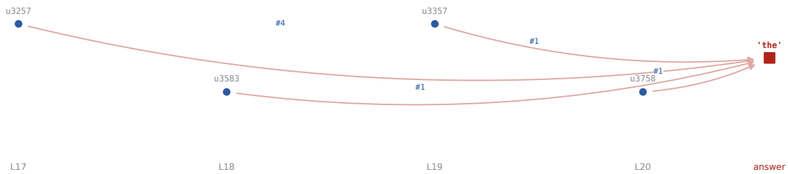
Figure 69: TinyLlama 1.1B, predictions 1 and 2. Of 20 predictions drawn at random, these are two of the four whose sufficient set is nearest the median, 5.
