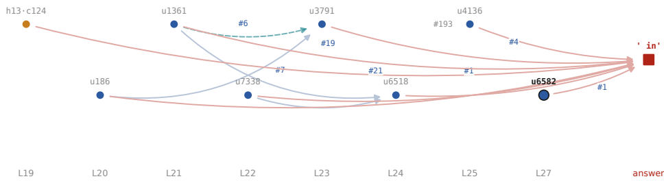
Figure 93: Llama-3.2 3B, prediction 4. Selected for containing edges no token describes. Of 20 predictions drawn at random, this is one of the four whose sufficient set is nearest the median, 8.
