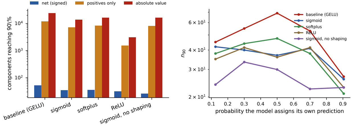
Figure 22: Left: the three denominators across the arms, on a log axis. The gap between the signed count and the other two is the same two-to-three orders of magnitude found in the baseline, and it is present in every arm — choosing the activation changes the size of the circuit, not whether the convention matters. Right: circuit size against how confident the model is in its own prediction. The arms keep their order at every confidence, so the comparison does not depend on where the confidence floor of Table 14 is set.
