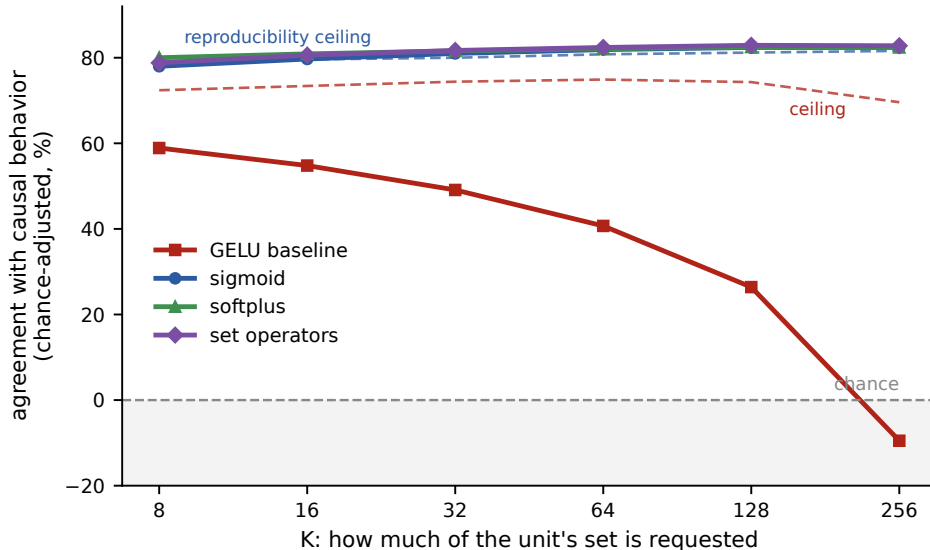
Figure 24: Agreement between the parameter-derived set and the causal set, against how much of the set is requested. The baseline curve is the one from Figure 7. The three arms built on order-preserving activations are flat in K and sit near the dashed reproducibility ceiling — the rate at which the causal measurement agrees with itself on independent contexts, which no reading procedure can exceed — and they land on each other. Set-operator agreement is taken on operand A . Context length 2048, candidate pool |V| = 512 , table and causal profile from 16 disjoint contexts each.
