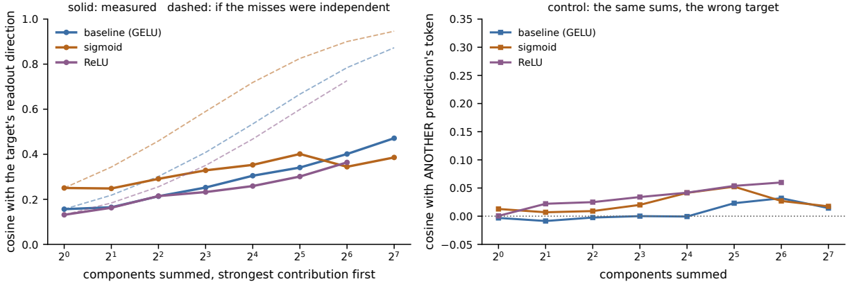
Figure 5: How a prediction is assembled. The cosine here is taken against a known target rather than searched for over the vocabulary, which is what makes it answerable where the column measures of Appendix C.11 are not. Left: the cosine between the target's readout direction and the running sum of what its components write, added strongest contribution first; the dashed line is the climb independent misses would give, anchored on each model's own first member. Every model falls below it, so the sum is carried by its largest terms rather than by their number. Right: the control, the same partial sums scored against a different prediction's token. Flat and near zero for every model plotted, so what the left panel shows is aim rather than undirected drift toward the token cone.
