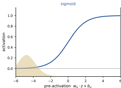
Figure 25: The sigmoid arm’s operating point, drawn on the same axes and to the same recipe as the baseline’s in Figure 20: the curve is the function and the shaded density under it is the measured distribution of pre-activations over a trained model of that arm. Its mass sits further left than the baseline’s, and it does not matter, because a monotone function preserves the ordering wherever its argument happens to land. It is not the operating point that causes the baseline’s reversal — it is that GELU has an interval where the ordering can be lost at all.
