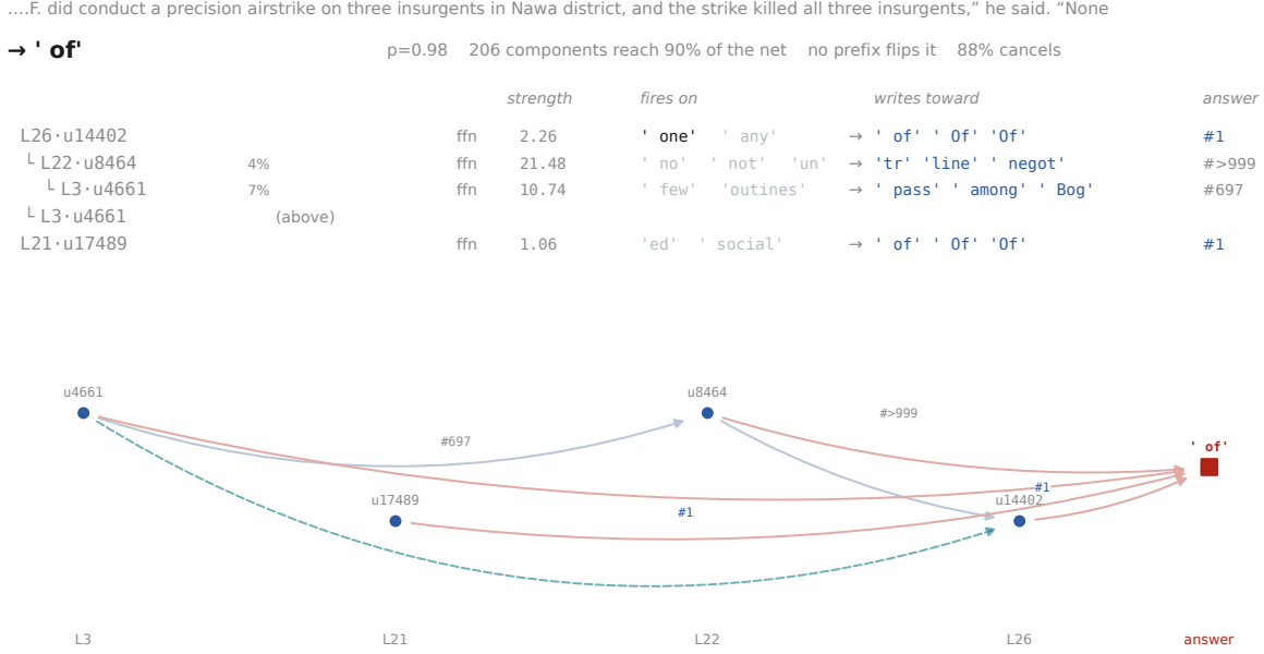
Figure 94: Qwen2.5 7B, prediction 4. Selected for containing edges no token describes. Of 17 predictions drawn at random, this is one of the four whose sufficient set is nearest the median, 4.
