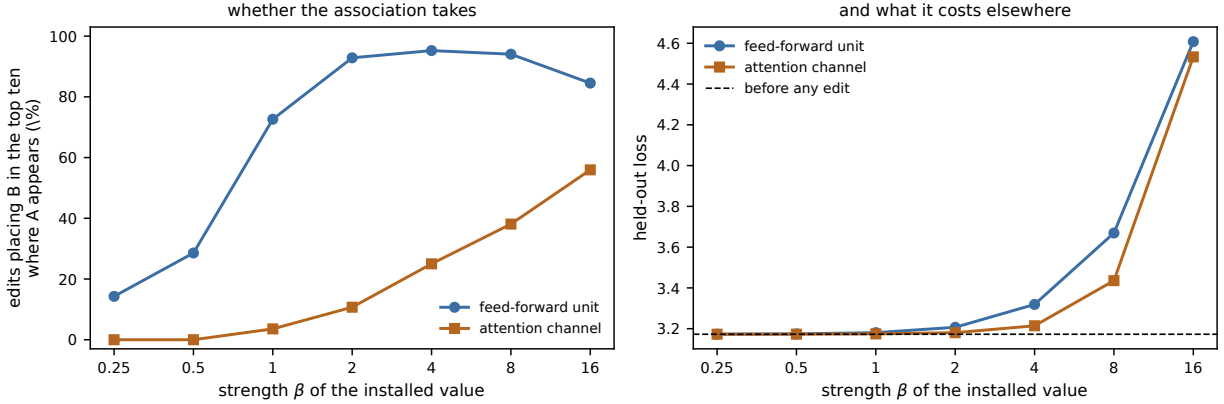
Figure 11: Left: how often the edit takes, against how hard it is pushed. A feed-forward unit takes it on nearly every trial from \beta = 2 upward, and at every depth through layer eight; an attention channel needs roughly eight times the strength and succeeds at scattered depths. Right: held-out loss against the same strength, with the unedited model dashed. The unit’s working range costs almost nothing and the channel’s does not.
