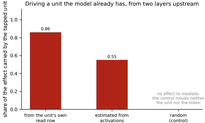
Figure 18: Share of the target’s promotion carried by the tapped unit, by how the driving direction was obtained, over twelve units per model at four write strengths. The random control moves neither the unit nor the target, so it has no effect to mediate.
