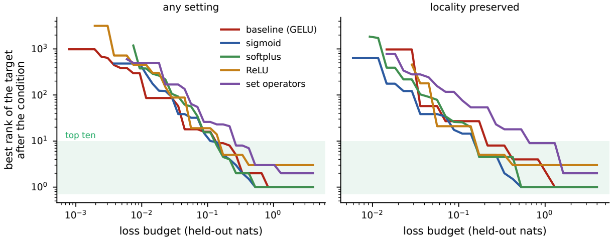
Figure 27: The best rank the target reaches for a given held-out loss budget, over the full cross of write strength, read gain, saturation, read-row calibration and marker tilt, with heads at layers four, six, eight, nine and ten reading at layer ten. Left: any setting. Right: the same with the specificity criterion imposed, so the target may not be promoted where it was not asked for. The gap between the panels is the price of specificity.
