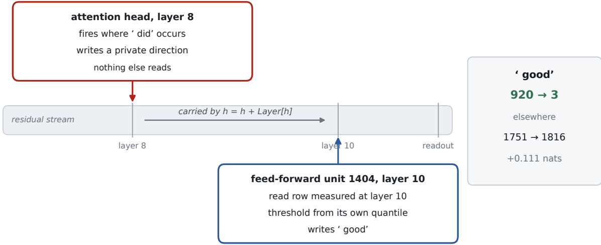
Figure 14: One installed pair, end to end. The head marks the positions, the stream carries the marker two layers without turning it, and the unit answers there. Ranks are for the target token at the positions the head fires on and at all other positions.
