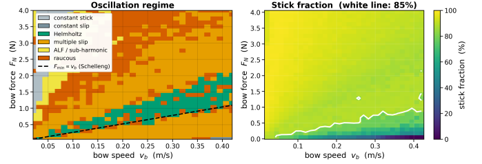
Fig. 2. Playability of the model. Left: oscillation regime, with the Schelleng minimum-bow-force trend overlaid. Right: stick fraction, the quantity that distinguishes Helmholtz motion from periodic slipping.
