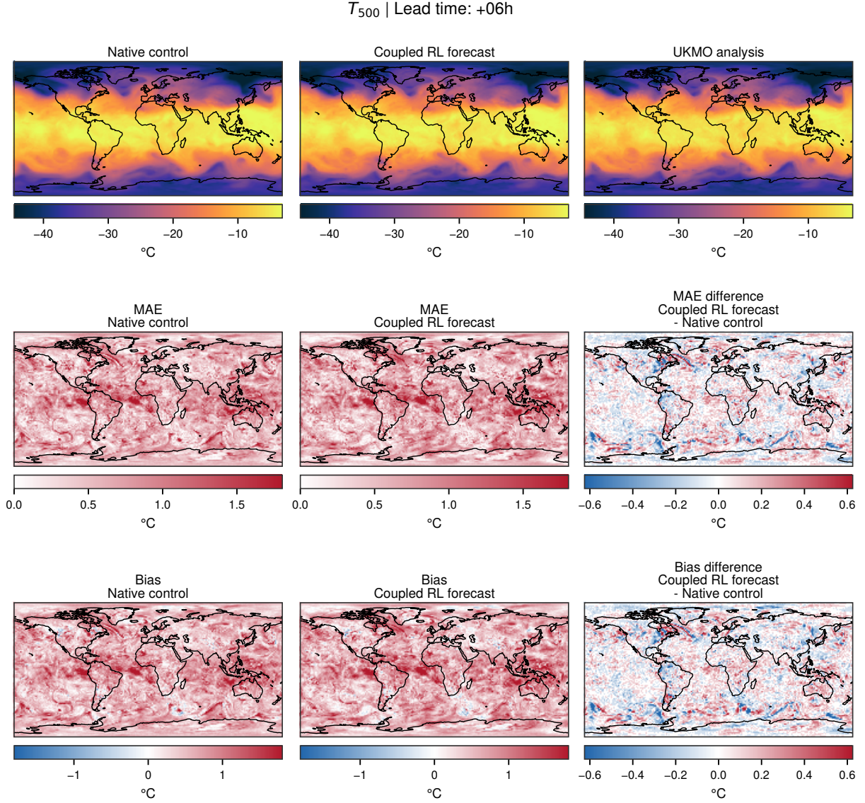
Figure D.3: T_{500} verification at +6 h. (a) The first row compares the native control, coupled RL forecast, and UKMO analysis. (b) The second row shows absolute error and its RL-minus-native difference. (c) The third row shows bias and its RL-minus-native difference. Blue values in the right-hand difference panels indicate a reduction relative to the native control, while red values indicate an increase. The T_{500} MAE increases in every latitude band, so this diagnostic provides an important counterexample to the Z_{500} improvement. Better geopotential-height verification therefore does not necessarily imply a corresponding improvement in temperature at the same pressure level.
