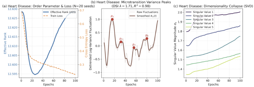
Figure 7: Heart Disease : Dimensionality collapse (c) is mirrored by a sequential 4-peak variance divergence ( \lambda = 1.71, R^2 = 0.98, \text{FPR} = 4.9\% ) mapping the internal topological constraints.
