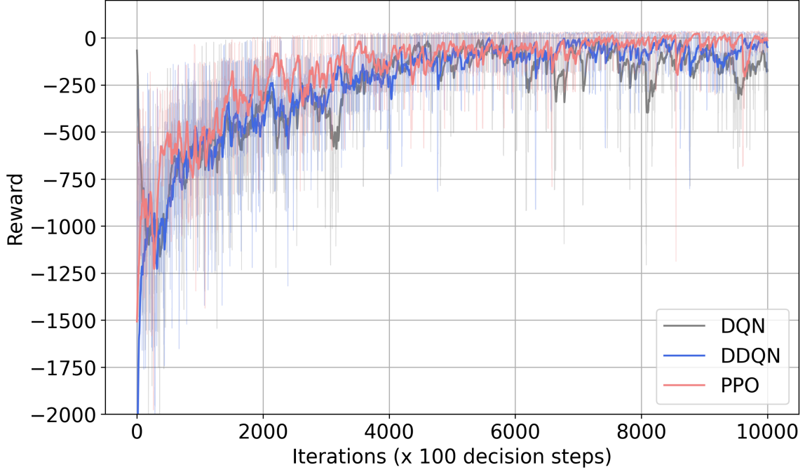
Figure 4: Reward evolutions
