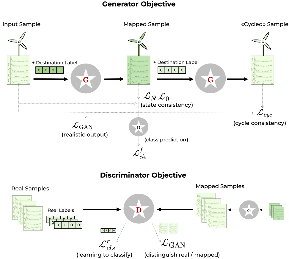
Figure 4: The generator objective is shown at the top. The generator is tasked to translate a sample to the specified destination domain. The adversarial loss forces the generator to output a realistic SCADA sample. It learns to match the destination domain through the classification loss obtained from the discriminator, while the two physics-informed state-consistency losses aim to preserve the operation by matching idle and maximum power states. The cycle-consistency loss directs the generator to map the translated sample back to its original input, enforcing further content preservation. The discriminator objective is shown at the bottom. The discriminator learns to classify real SCADA samples to their corresponding domain and to distinguish between real and mapped samples.
