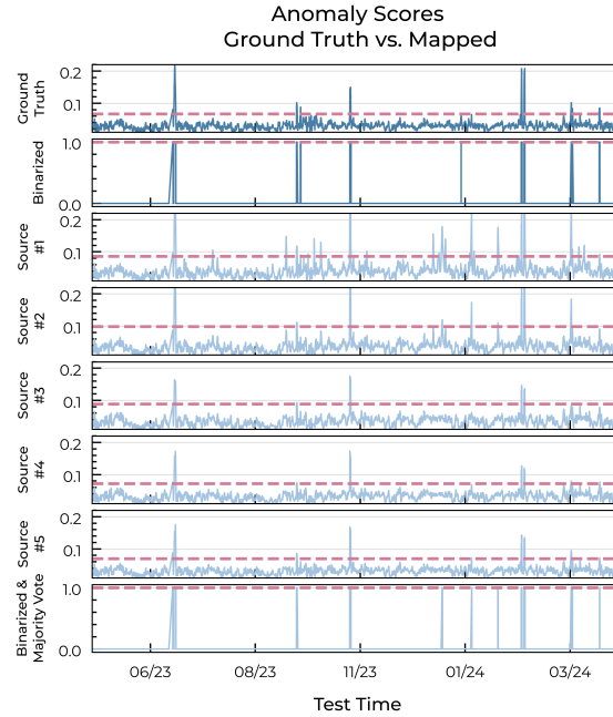
Figure 11: Anomaly scores for test data of target WT05 (setup 5). The ground truth (top) is compared samples mapped to and scored in each source domain. The model was trained on 3 weeks of target data.
