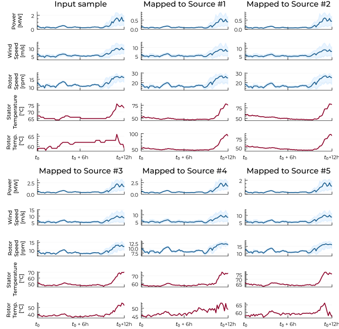
Figure 10: An input sample of target WT05 mapped to each source domains (setup 5). The model was trained on 3 weeks of target data.
