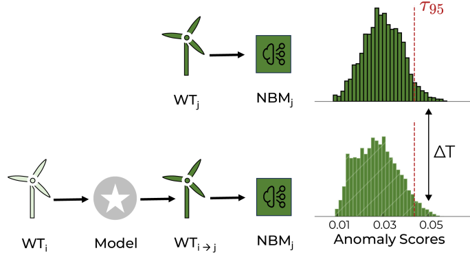
Figure 6: The proxy metric \Delta_T is calculated by comparing the tail of anomaly scores of real validation data (top) and mapped anomaly scores (bottom).
