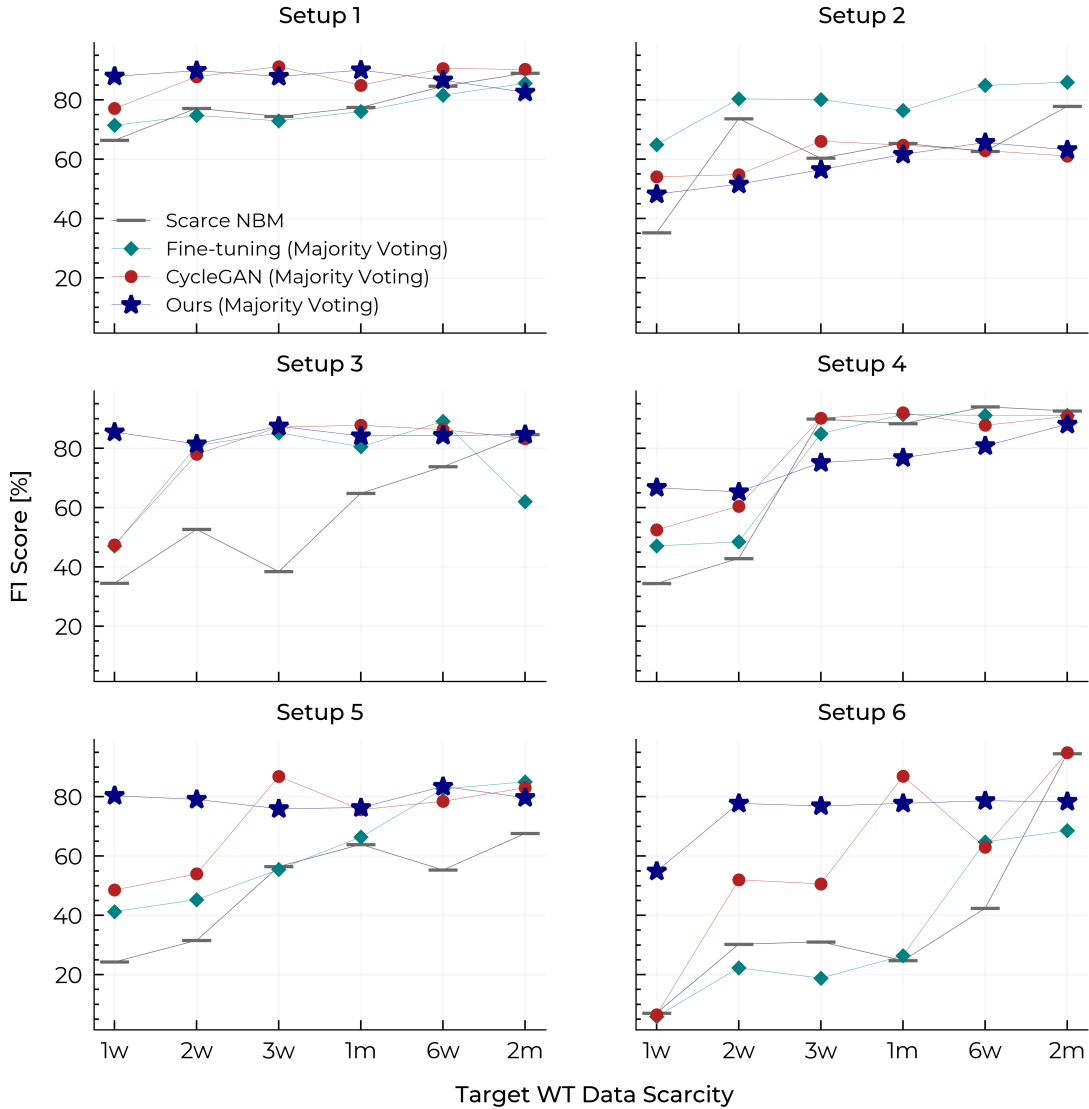
Figure 8: F1 scores showing the similarity of model scores to the ground truth for all setups and data scarcity scenarios.
