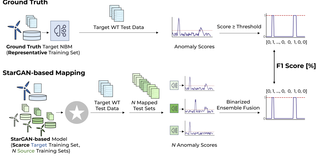
Figure 5: The ground truth anomaly scores are shown at the top. An NBM trained on representative target WT training data evaluates target test samples and yields anomaly scores that are subsequently binarized. We assess the fault detection of our model by mapping target test samples to all source domains for evaluation with their NBMs, before they are binarized and fused, as shown at the bottom. The F1 score is calculated between the binarized ground truth and the fused binarized model scores.
