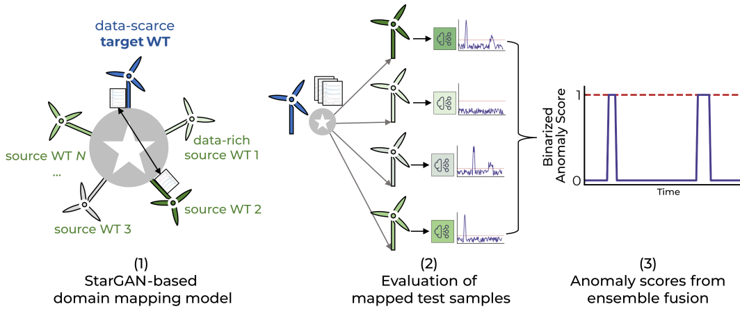
Figure 3: A visual summary of our proposed approach. (1): A StarGAN model is trained to map SCADA samples across several source WTs and a target WT. (2): At inference time, target WT test data is mapped to all source WTs and evaluated with their corresponding pretrained NBMs. (3): Anomaly scores are binarized and combined using an ensemble fusion strategy to obtain the final scores.
