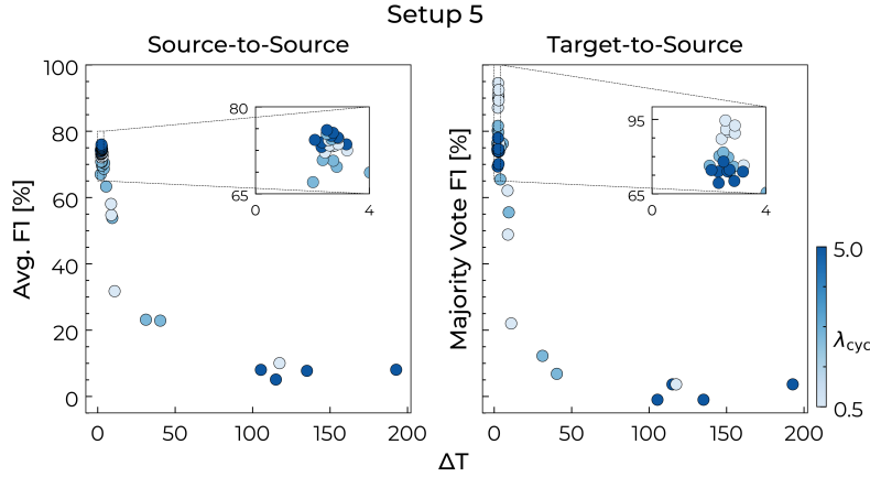
Figure 9: \Delta_T of 36 different model candidates in comparison to the average F1 score when mapping data-rich source WTs to each other (left) and the F1 score with majority vote ensemble fusion when mapping the target WT to all source WTs. Results are shown for the model selection performed for setup 5 under 1 month of target WT data scarcity.
