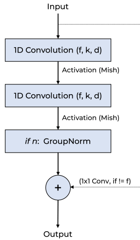
Figure A1: Residual block architecture, as used in [5].
