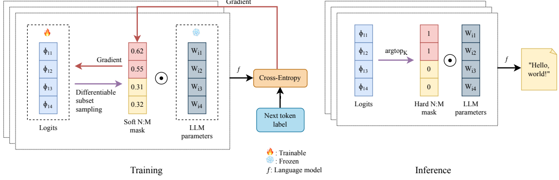
Figure 2: Overview of the RoI framework for semi-structure sparsity learning via differentiable subset sampling, illustrating the training and inference phases.
