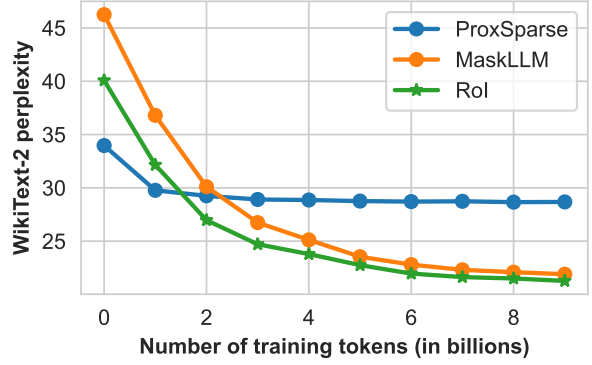
Figure 3: RoI demonstrates better scalability than MaskLLM and ProxSparse, with WikiText-2 perplexity (on the Qwen2.5-1.5B model) improving more consistently as the number of training tokens increases.
