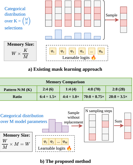
Figure 1: Learnable semi-structured N:M sparsity methods: a) modeling the mask selection process using a categorical distribution over feasible masks, and b) our proposed method by learning to sample subsets without replacement of model parameters. The proposed method is more memory efficient than previous works for most practical N:M sparsity patterns. The memory advantage becomes more pronounced as M increases or when N is around M/2 .
