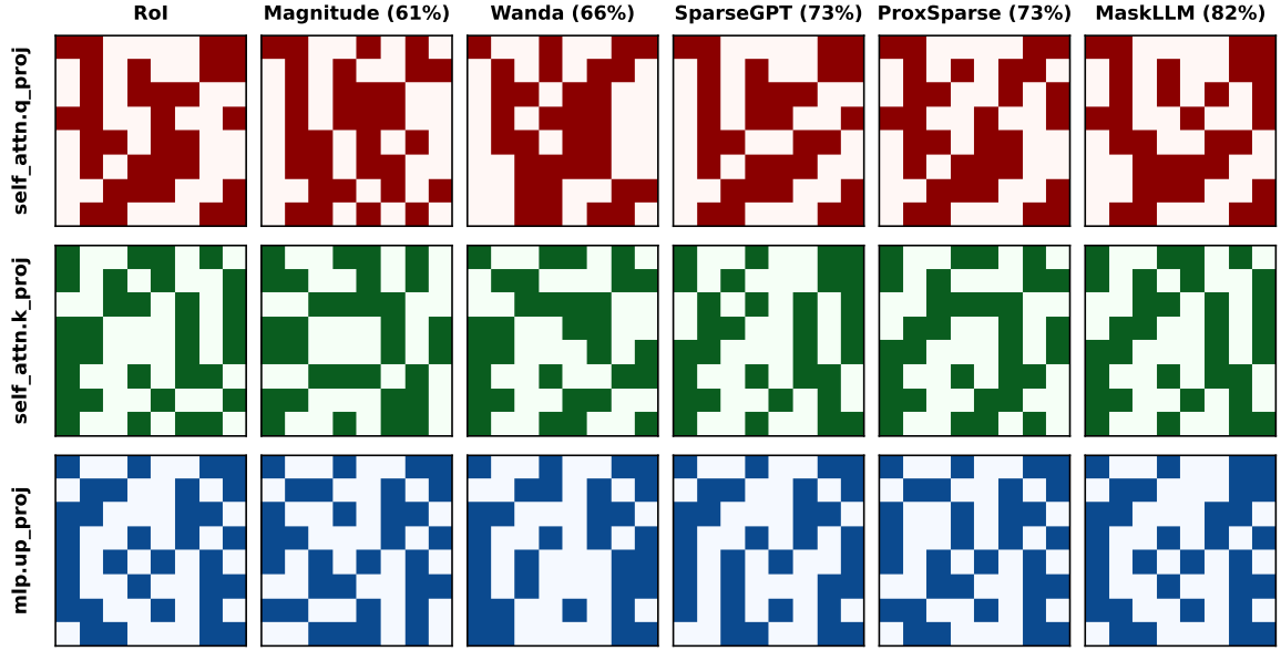
Figure 4: Mask difference comparison between RoI and previous works on the Qwen2.5-7B model. Besides the name of each baseline, place an overlapping percentage indicating the similarity of the produced masks between that baseline and RoI. Bold pixels indicate masks corresponding to retained weights.
