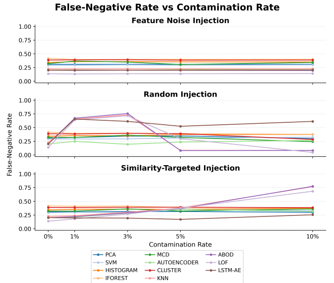
Fig. 3. FNR versus training-pool-relative contamination budget. LOF, KNN, ABOD, and LSTM-AE enter the highest missed-detection region under one or more injection settings.
