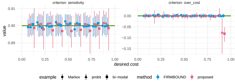
(b) Constraints on sensitivity (left) and cost (right) are satisfied by the proposed method.
