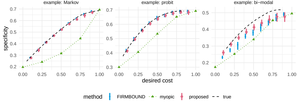
(a) Specificity achieved by different methods at varying monitoring-cost levels.
