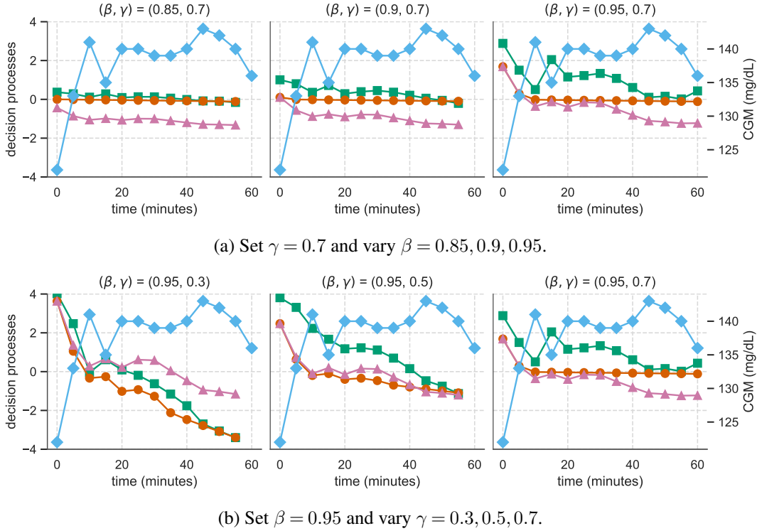
Fig 4.5: Effects of different sensitivity ( \beta ) and cost ( \gamma ) constraints on the decision processes for the non-hypoglycemia CGM trajectory (Figure 4.3c).
