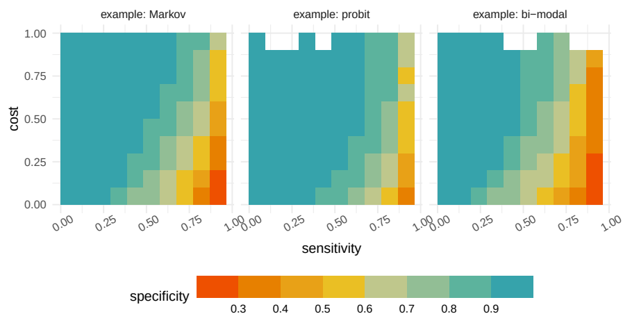
Fig 4.2: The operating characteristic heatmaps of the sequential rules illustrates the three-way trade-off among specificity, sensitivity, and cost. Each tile represents the binned and averaged performance over 50 repeated experiments.
