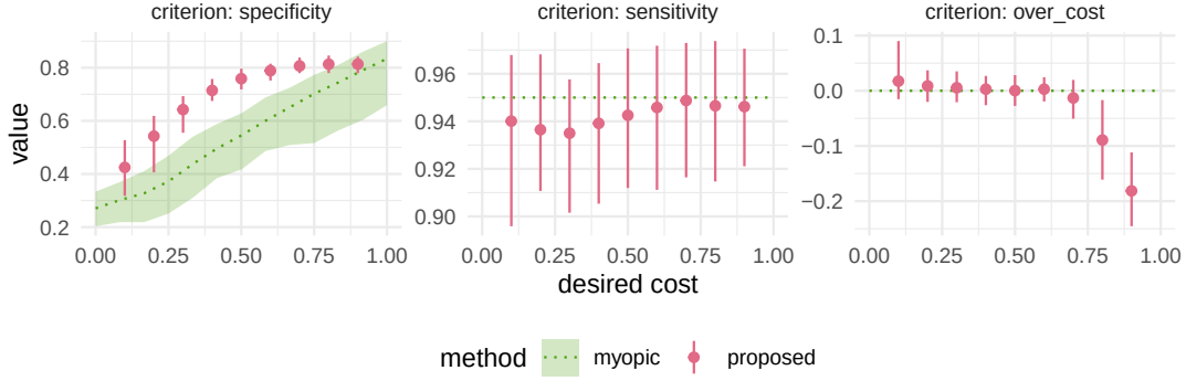
Fig 4.4: Performance of the proposed sequential decision rules and the myopic baseline under a sensitivity constraint of \beta = 0.95 across cost \gamma = 0.1, \dots, 0.9 . The leftmost panel illustrates the specificity–cost trade-off under the sensitivity constraint. The middle and rightmost panels examine whether the constraints were satisfied; the over cost (the rightmost panel) is defined as the achieved cost minus the desired cost. Means (dots) and 90% intervals (bars and ribbons) are shown over 50 repeated cross-validation experiments. To reduce visual clutter, the dots and bars for the myopic baseline are replaced with dotted lines and ribbons.
