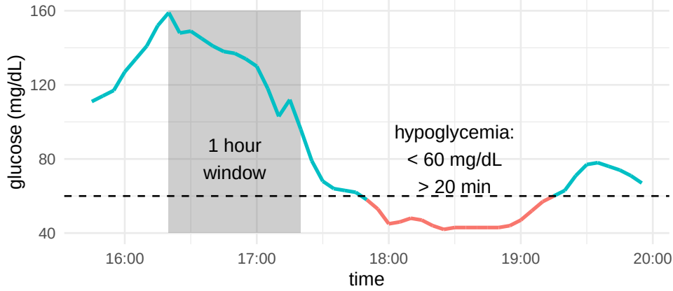
(a) An example one-hour monitoring window (shaded), followed by a hypoglycemia episode within 30 minutes.
