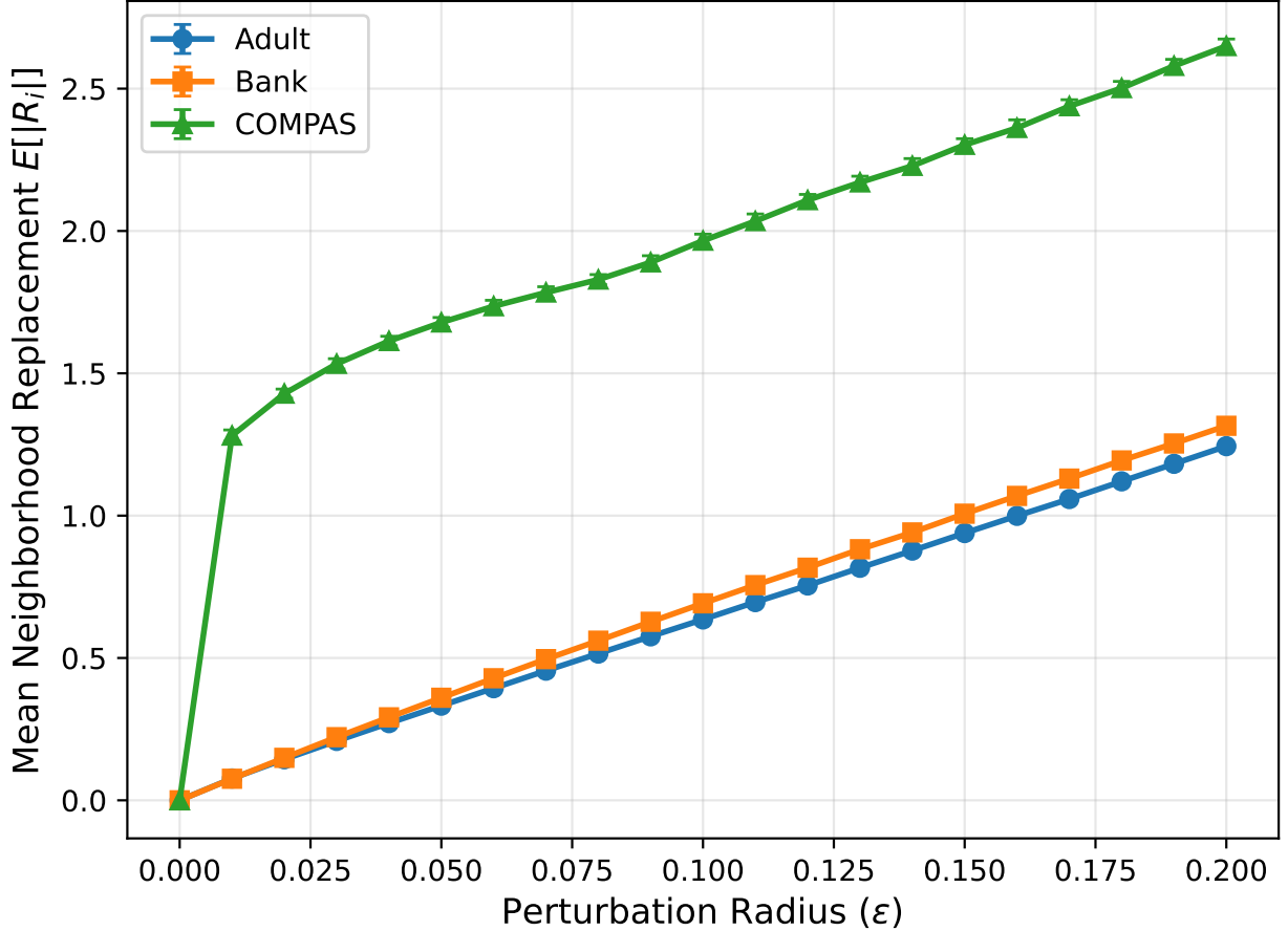
Figure 2: Expected neighborhood replacement \mathbb{E}[|R_i|] as a function of the perturbation radius \epsilon . Neighborhood replacement increases monotonically across all datasets, with COMPAS exhibiting substantially greater geometric sensitivity than Adult and Bank.
