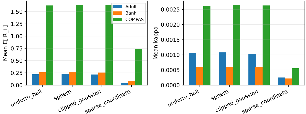
Figure 3: Neighborhood replacement (left) and audit volatility (right) under four perturbation models with identical perturbation budgets. Despite differences in the perturbation distributions, audit volatility consistently follows neighborhood replacement across all datasets.
