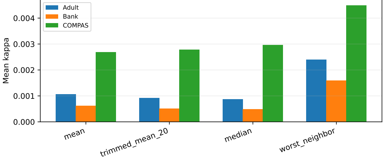
Figure 5: Audit volatility under different aggregation operators. Robust aggregators (trimmed mean and median) consistently exhibit lower volatility than the worst neighbor operator, supporting Theorem 6.
