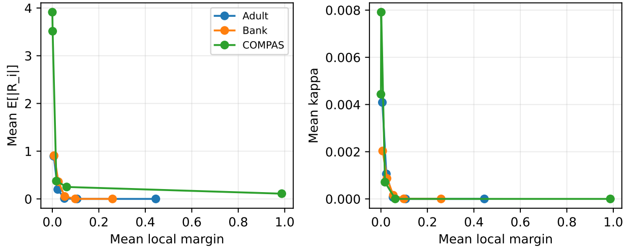
Figure 6: Effect of the local separation margin on audit robustness. Left: Expected neighborhood replacement \mathbb{E}[|R_i|] decreases with increasing separation margin. Right: Audit volatility \kappa exhibits the same trend, approaching zero for well-separated neighborhoods.
