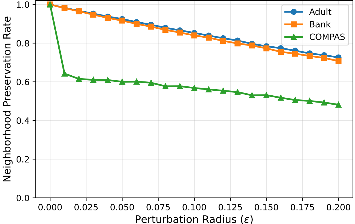
Figure 1: Neighborhood Preservation Rate (NPR) as a function of the perturbation radius \epsilon . Larger perturbations progressively reduce neighborhood stability, consistent with Theorem 3.
