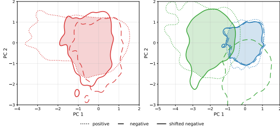
Figure 3: Activation-space view on Llama2 7B, layer 26, head 4, under PCA. Left : ITI shifts every negative point along a single mass-mean direction, producing one shifted distribution (red, solid) that lands inside the positive support but only covers part of it. Right : cluster-based steering with n_c = 2 splits the negative cloud into two sub-modes (blue, green) and applies a separate direction to each. The two shifted clusters together cover the positive support more completely.
