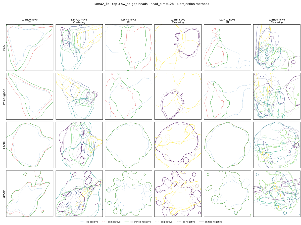
Figure 7: Llama2 7B, top-3 heads by sw_hd gap, under four projection methods (rows). Each pair of columns shows ITI and clustering for one head.
