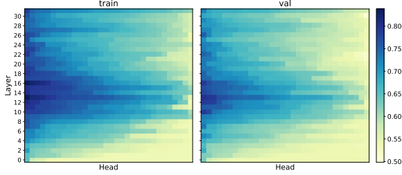
Figure 2: Per-head truthfulness probe accuracy on Llama2 7B. Left: train split. Right: held-out val split.
