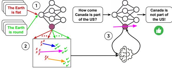
Figure 1: IDEAA framework for input-dependent steering. (1) Collects per-head activations from contrastive prompts. (2) Clusters the positive (green) and negative (red) supports (Sec. 4.1) and obtains the cluster-optimal direction vectors (Sec. 4.2). (3) Finds the direction that best aligns with the input (pink), and use that for steering (Sec. 4.3).
