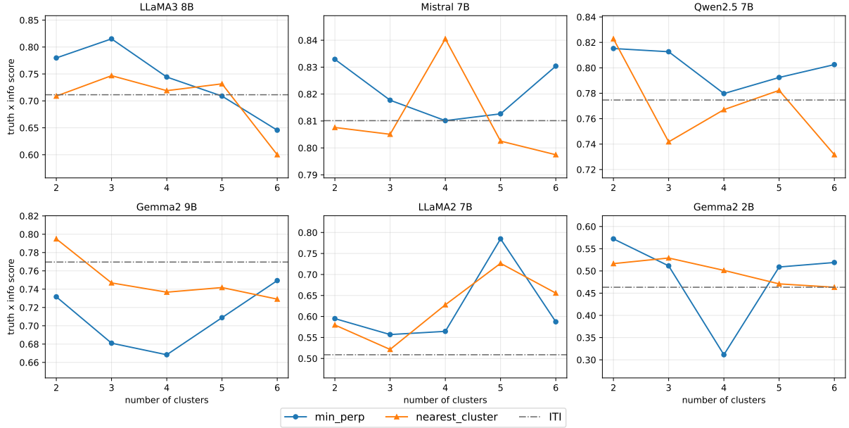
Figure 5: Effect of n_c across all six models. Each subplot mirrors Figure 4: truth \times info rate for the best (K, \alpha) at each n_c for min-perp and nearest-cluster.
