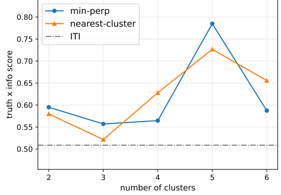
Figure 4: Effect of n_c on Llama2 7B. Each point is the best \text{truth} \times \text{info rate} over (K, \alpha) for a given n_c . Both min-perp and nearest-cluster are consistently above ITI.
