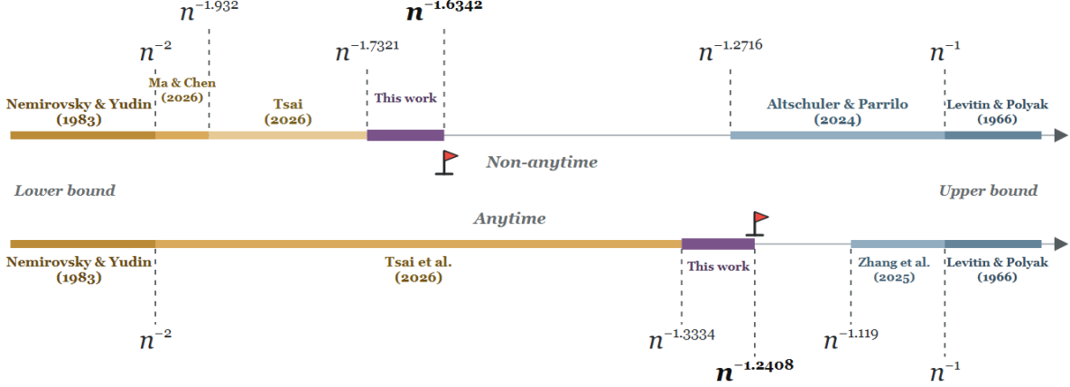
Figure 1: Improved lower bounds for GD.
