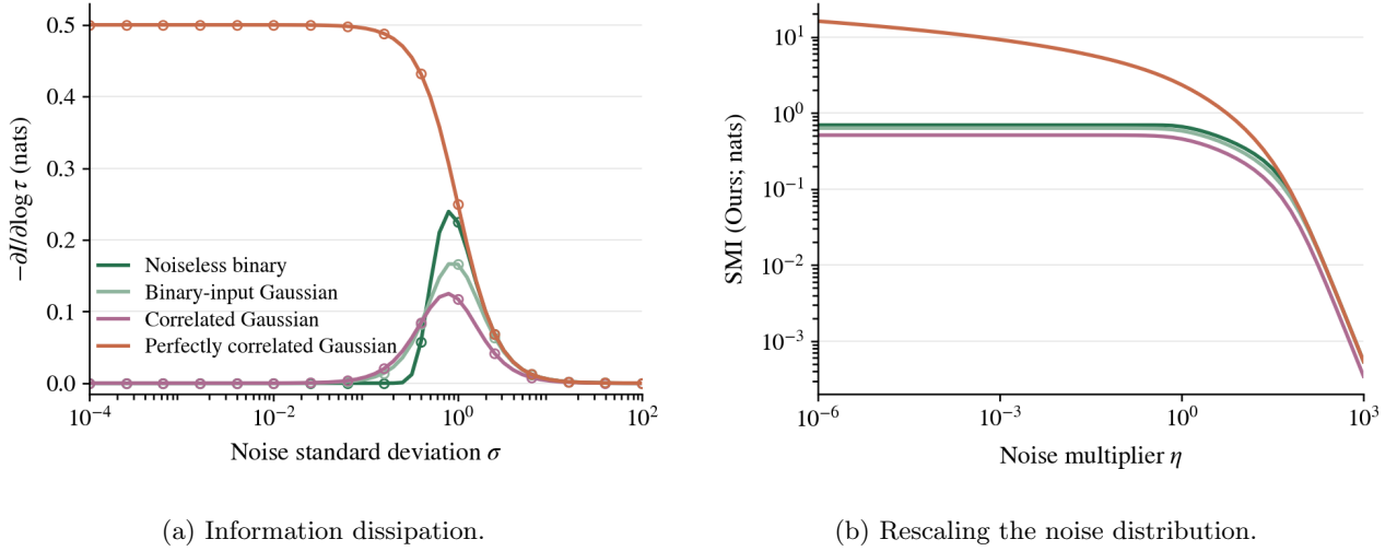
Figure 10: Information across noise levels. Exact-density evaluations. (a) \frac{\tau}{2}\mathbb{E}[v_\tau^2] (lines) and -\partial I/\partial \log \tau (markers), with \tau = \sigma^2 . (b) Multiscale SMI for \sigma \sim \text{LogUniform}(0.01\eta, \eta) .
