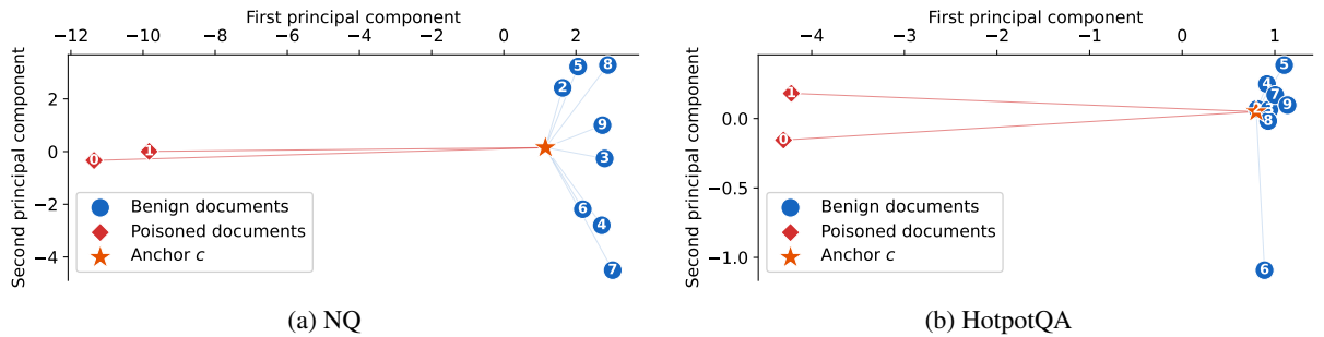
Figure 3: Poisoned documents are geometric outliers in the topic-removed residual space with ten retrieved documents including two injected poisoned documents. NQ query: “who played miss wheeler in carry on teacher”; HotpotQA query: “The mass killing that took place at Oakland, California on April 2, 2012 was less deadly than the one that took place on October 1, 2015 in which state?” ● benign, ◆ poisoned, ★ geometric median anchor c .
