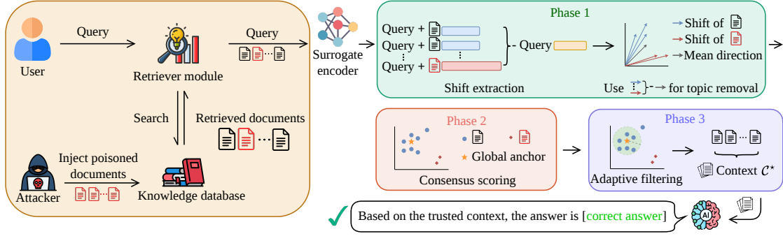
Figure 4: Overview of the RAGSentinel pipeline. An attacker injects poisoned documents into the knowledge database (left). The surrogate encoder encodes each query-document pair and extracts hidden-state shifts (Phase 1). Consensus scoring identifies poisoned documents as geometric outliers via the global anchor (Phase 2). Adaptive filtering keeps a trusted context C^* (Phase 3), which is passed to the black-box LLM for answer generation.
