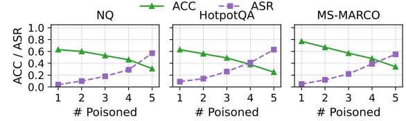
Figure 2: Impact of the number of poisoned documents on RAGSentinel under PoisonedRAG.
