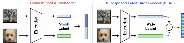
Figure 1: AE vs. SLAE at matched storage. SLAE shares wider latent representations through superposition instead of shrinking each latent independently.
