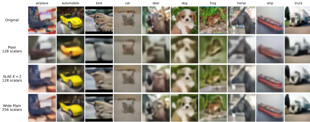
Figure 8: Qualitative reconstructions on CIFAR-10. Reconstructions at H = 2 and K = 2 . Plain AE and SLAE both use an average storage budget of 128 scalars per example. Wide Plain uses the same wide latent geometry as SLAE but stores each latent independently and therefore requires 256 scalars per example.
