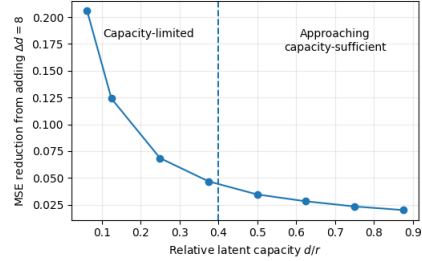
Figure 2: Adding latent width ( \Delta d = 8 ) yields the largest reconstruction gain when the autoencoder is capacity limited, with diminishing benefit as d/r grows. The dashed line qualitatively separates the two regimes.
