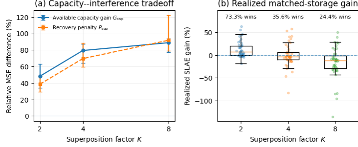
Figure 5: Capacity–interference tradeoff as superposition increases. Results use the same 45 (dataset, H , B ) configurations for all K \in \{2, 4, 8\} . Left: median capacity gain G_{\text{cap}} and recovery penalty P_{\text{sup}} , with interquartile ranges. Right: distribution of the realized matched-storage gain \Delta_{\text{SLAE}} = G_{\text{cap}} - P_{\text{sup}} ; positive values indicate an improvement over Plain.
