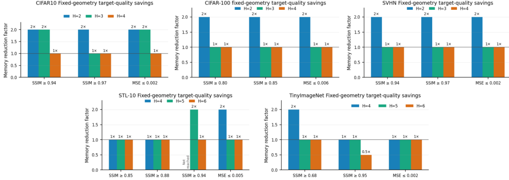
Figure 14: Fixed-geometry memory efficiency at matched reconstruction quality. For each dataset and latent spatial size H , we report the ratio of the minimum evaluated Plain AE storage budget to the minimum evaluated SLAE storage budget required to reach each target quality. Values above 1\times indicate an SLAE memory saving, 1\times indicates parity, and values below 1\times indicate that SLAE requires more storage. Quality targets are selected separately for each dataset to reflect its observed reconstruction range.
