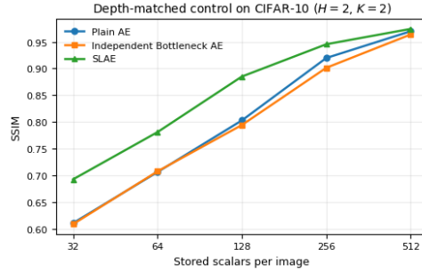
Figure 6: Depth-matched control. CIFAR-10, H = 2 , K = 2 . The Independent Bottleneck AE adds comparable compression machinery but stores examples independently.
