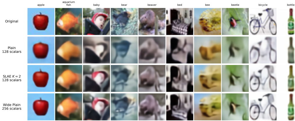
Figure 9: Qualitative reconstructions on CIFAR-100. Reconstructions at H = 2 and K = 2 . Plain AE and SLAE are matched at 128 stored scalars per example, while Wide Plain uses the corresponding wider latent independently and requires 256 scalars per example.
