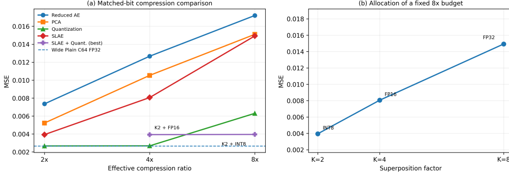
Figure 15: Alternative latent-compression strategies on CIFAR-10. We use H = 2 and a C = 64 Wide Plain FP32 latent as the reference. (a) Reconstruction MSE under matched per-image latent-memory bit budgets. SLAE outperforms dimensional compression through both reduced-width autoencoders and PCA, while numerical precision reduction is highly effective at mild compression. At 8\times , combining K = 2 superposition with INT8 shared-memory storage achieves the lowest MSE with 37.3% reduction relative to the strongest INT4 quantization at the same bit budget. (b) Allocation of a fixed 8\times compression budget between superposition and numerical precision. Moderate K = 2 superposition with INT8 storage substantially outperforms allocating more of the compression to superposition.
