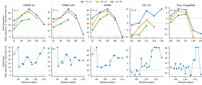
Figure 4: Reconstruction improvement at matched latent storage. Relative MSE reduction of SLAE over Plain at the same average number of stored scalars per example. Top: controlled fixed-geometry comparison for K \in \{2, 4, 8\} . Bottom: global best-under-budget comparison, where each method selects its best available latent configuration. Positive values indicate an SLAE improvement. Lines in the bottom row connect independently selected configurations only as a visual guide. Y-axis limits vary across datasets for readability.
