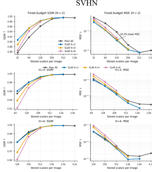
Figure 12: Full reconstruction results on SVHN. Fixed-geometry SSIM and MSE curves for H \in \{2, 3, 4\} at matched average latent storage for K \in \{2, 4, 8\} .
