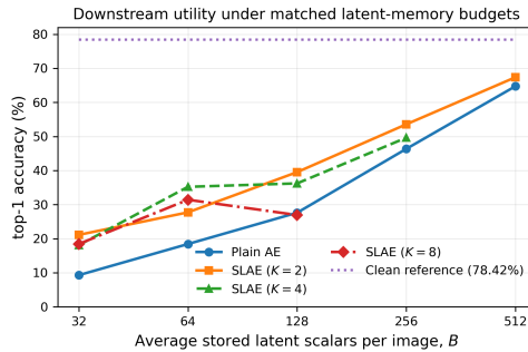
Figure 7: Downstream utility at matched storage. CIFAR-100 top-1 accuracy when the same CIFAR-style ResNet-18 is trained on Plain AE or SLAE reconstructions and evaluated on the same clean test set.
