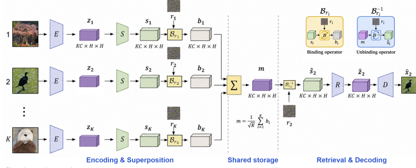
Figure 3: SLAE Architecture. Each input x_i is encoded by E into a wide latent z_i , transformed by the storage adapter S into s_i , bound with a slot-specific key r_i , and superposed with the other codes into shared memory m . Retrieval applies the corresponding inverse binding to obtain \hat{s}_i , which the recovery network R maps to a decoder-friendly latent \hat{z}_i for reconstruction by D . SLAE thus enables multiple wide latents to share the same memory through learned storage and recovery.
