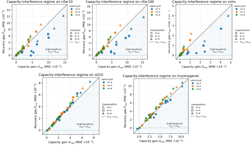
Figure 13: Dataset-wise capacity–interference decomposition. Each point represents a matched-storage operating point. The horizontal axis shows the capacity gain G_{\text{cap}} obtained from the corresponding K -times-wider Plain AE, and the vertical axis shows the recovery penalty P_{\text{sup}} incurred by SLAE relative to that wide representation. Points below the dashed line P_{\text{sup}} = G_{\text{cap}} correspond exactly to settings in which SLAE improves over the matched-storage Plain AE. Colors indicate latent spatial size H , while marker shapes indicate K \in \{2, 4, 8\} .
