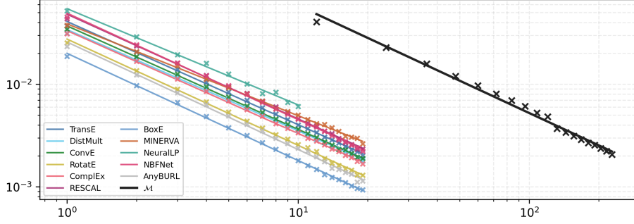
Fig. 6: Power-law fits of \Delta\text{MRR}(k) (y-axis) w.r.t. instance number (x-axis) in log-log scale across models on FB15k-237.
