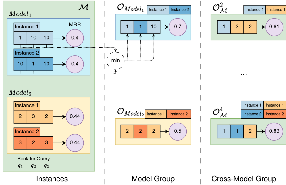
Fig. 1: Per-query selection mechanism of oracles. Although individual instances achieve similar aggregate MRR, their performance differs at the query level ( q_1, q_2, q_3 ). By selecting the best rank per query across instances, the oracle constructs optimal pseudo-instances at the model group level ( \mathcal{O}_{Model} ) and cross-model group level ( \mathcal{O}_{\mathcal{M}} ), leading to higher overall performance.
