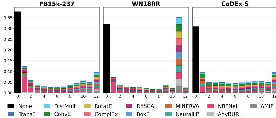
Fig. 3: Distribution of queries according to the number of model oracles achieving Hit@1
