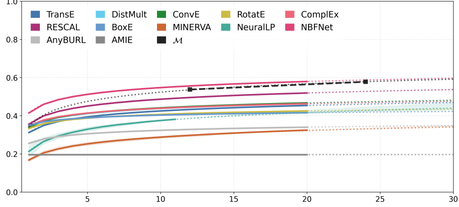
Fig. 5: Evolution of oracle MRR as a function of the number of instances k on FB15k-237.
