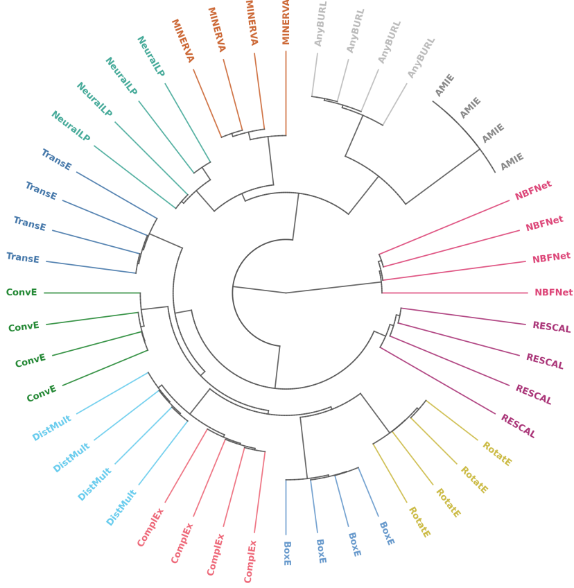
Fig. 4: Dendrogram of instance similarities on FB15k-237.
