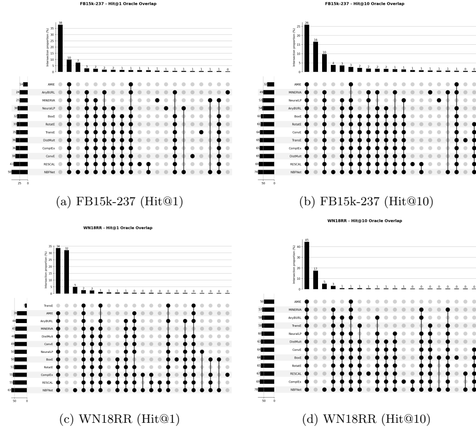
Fig. 7: UpSet plots showing the distribution of correctly answered queries across the 20 most frequent combinations of models for FB15k-237 and WN18RR. Each bar represents the proportion of queries solved by a specific subset of models, enabling the analysis of overlap and model complementarity at different evaluation thresholds (Hit@1 and Hit@10).
