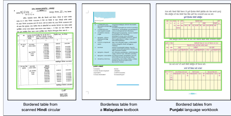
Fig. 2: Sample images from MANDALA with tables in bounding boxes.
