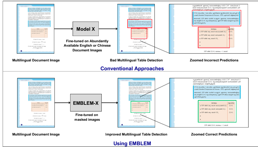
Fig. 1: Comparative analysis of conventional TD approaches and improvement brought through our method, EMBLEM, on a Malayalam document page.
