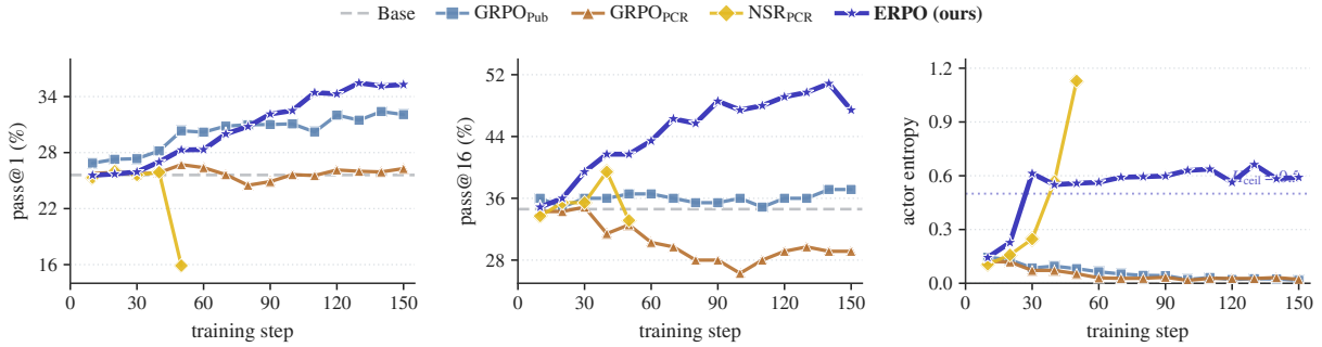
Figure 4: Per-step training dynamics on Qwen3-8B / LiveCodeBench. Left: pass@1. Middle: pass@16. Right: actor policy entropy. Dashed gray lines mark the Base reference. The dotted indigo line marks ERPO’s fixed entropy ceiling H_{\text{ceil}} = 0.5 . NSR PCR is shown through step 50 because its entropy subsequently diverges and validation pass@k collapses.
