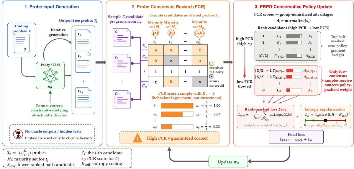
Figure 2: Overview of ERPO. Our method has three stages: (1) generating output-free probe inputs for each problem; (2) executing sampled candidates on the shared probes and scoring them by behavioral agreement (PCR); (3) a rank-masked, entropy-regularized update that uses PCR primarily to suppress low-consensus candidates.
