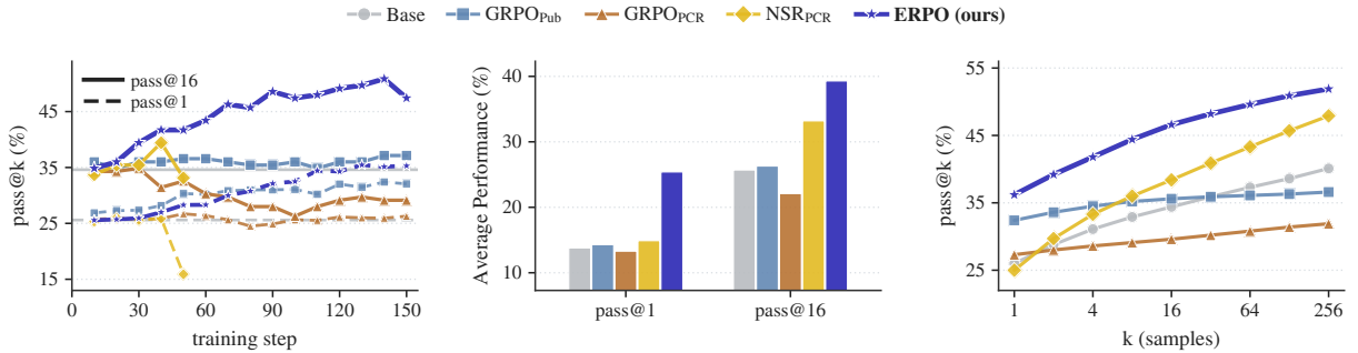
Figure 1: Performance overview. Left: Qwen3-8B per-step LCB results. Middle: Qwen3-4B mean transfer performance across three target benchmarks. Right: Qwen3-4B LCB inference-time scaling.
