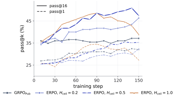
Figure 3: Entropy ceiling ablation on LiveCodeBench.
