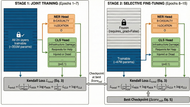
Fig. 3. Two-stage training procedure. Stage 1 (epochs 1–7) trains all layers jointly. Stage 2 (epochs 8–15) freezes layers 1–18 and fine-tunes only the upper six layers and task heads, reducing active parameters from 355M to 47M.
