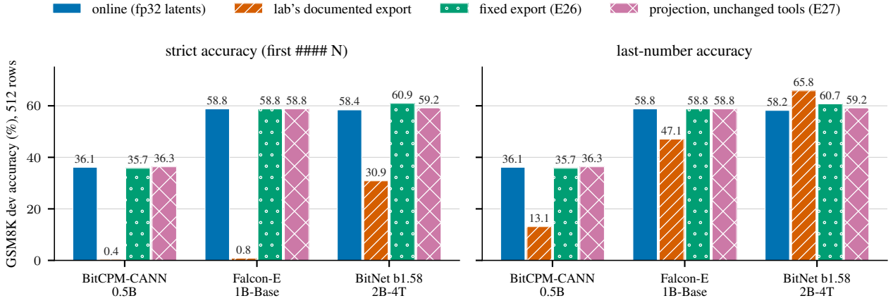
Figure 1. GSM8K dev accuracy (512 rows, greedy) of one fine-tuned endpoint per model: evaluated online from the fp32 latents, after the lab’s documented export, after the fixed export (Experiment 26) and after the projection that lets the unchanged tools emit the online codes (Experiment 27). Strict accuracy takes the first ##### N; the last-number rule takes the last number. The documented paths differ by model (§4). Bars are descriptive point estimates; the paired contrasts and their intervals are in Tables 3 and 4.
