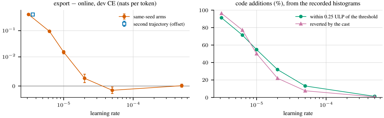
Figure 3. Falcon-E-1B-Base, the documented export across fine-tuning learning rates (fp32 latents, one trajectory per arm). Left: export minus online dev cross-entropy with 95% paired row-bootstrap intervals, on a symmetric log scale; the open square is the second trajectory at the lowest rate, offset horizontally for visibility. Right: descriptive summaries of each endpoint’s recorded margin histogram, the share of code additions within 0.25 bf16 ULP of the threshold and the share the cast reverts; they are counts, not measurements of latent displacement. Lines connect the declared rates for reading; no curve or between-rate difference was tested.
