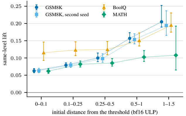
Figure 4. Same-level lift (the crossers’ share of positive first-order scores minus their level-mates’ share) by initial distance from the threshold on 2B-4T, at the GSM8K endpoint, its second seed, and the BoolQ and MATH endpoints. Bars are 95% tensor-bootstrap intervals conditional on each endpoint; only bins with at least 1,000 crossers from at least 10 tensors are drawn.
