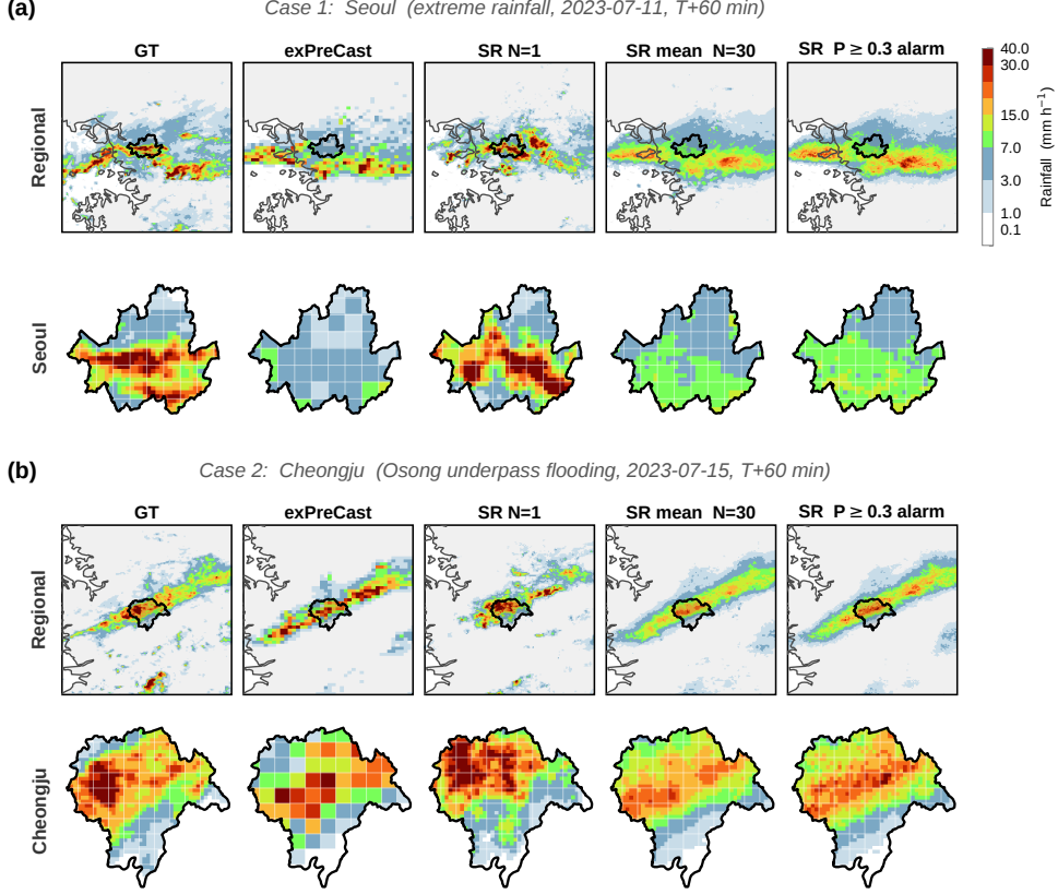
Fig. 5 City-scale case studies. (a) Case 1, Seoul extreme rainfall (2023-07-11, T+60 min); (b) Case 2, Cheongju underpass flooding (2023-07-15, T+60 min). For each case the top row is the regional view and the bottom row zooms to the city, with the city boundary outlined. Each row compares the ground truth, the exPreCast backbone, a single SR member, the 30-member SR mean, and the alarm mask. In (a) the single member shown is one that places the rainband over central Seoul; members differ in the position of the band. The SR mean and the alarm panel use all 30 members. The backbone is at 4 km and the SR outputs at 1 km. The alarm panel is not a binary mask: each pixel is colored by the highest level of the shared rainfall scale that at least 30% of the members exceed, so it can be read against the other columns directly. Thresholding this panel at a given level recovers the binary alarm mask M_{\text{alarm}} of Section 4.2 at that level.
